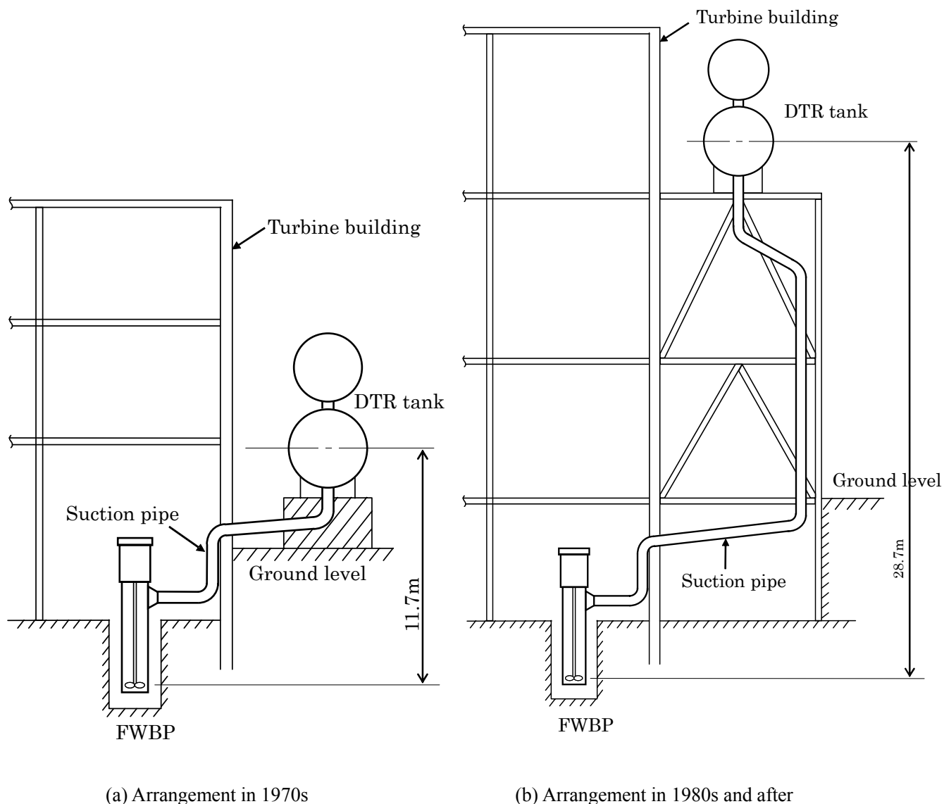
Fig. 4.4 The arrangement of DTR-tank and FWBP
