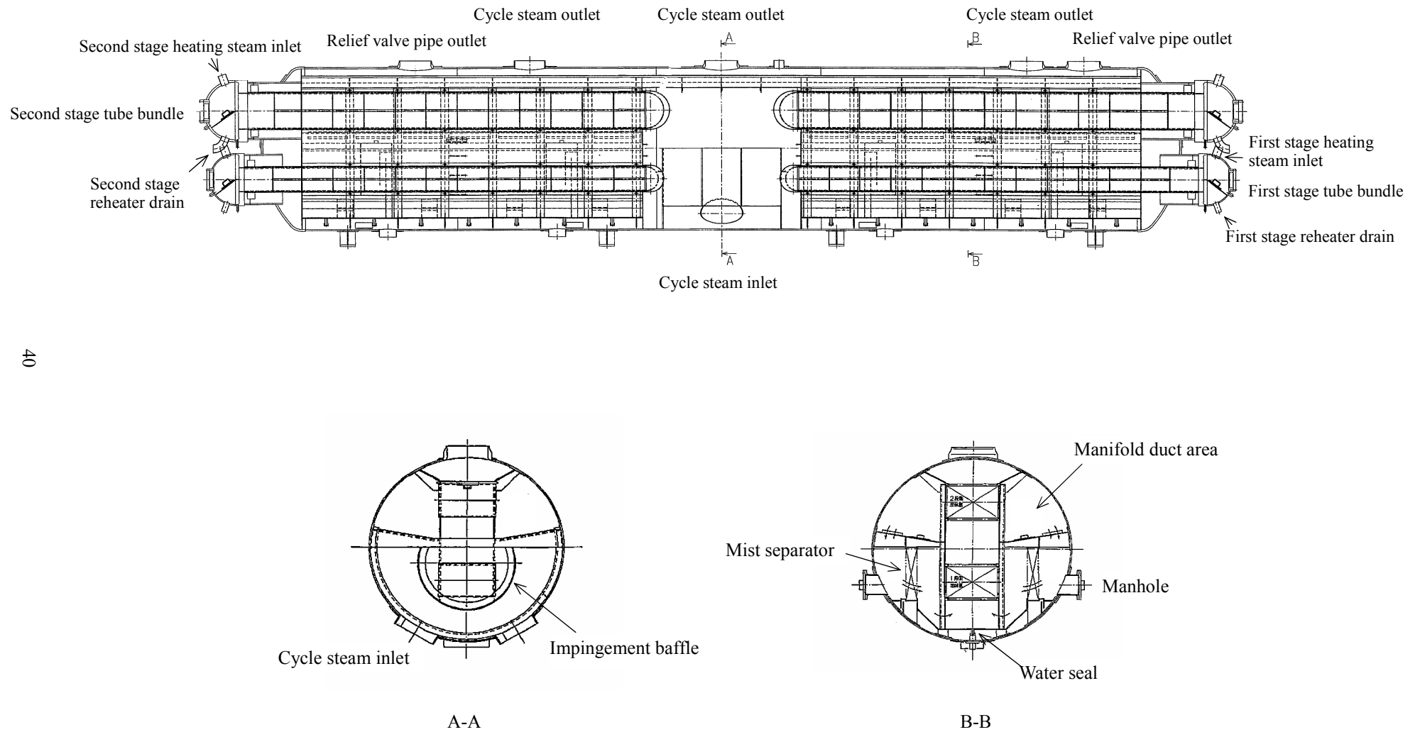
Fig. 2.6 Current model MSR in Japan
