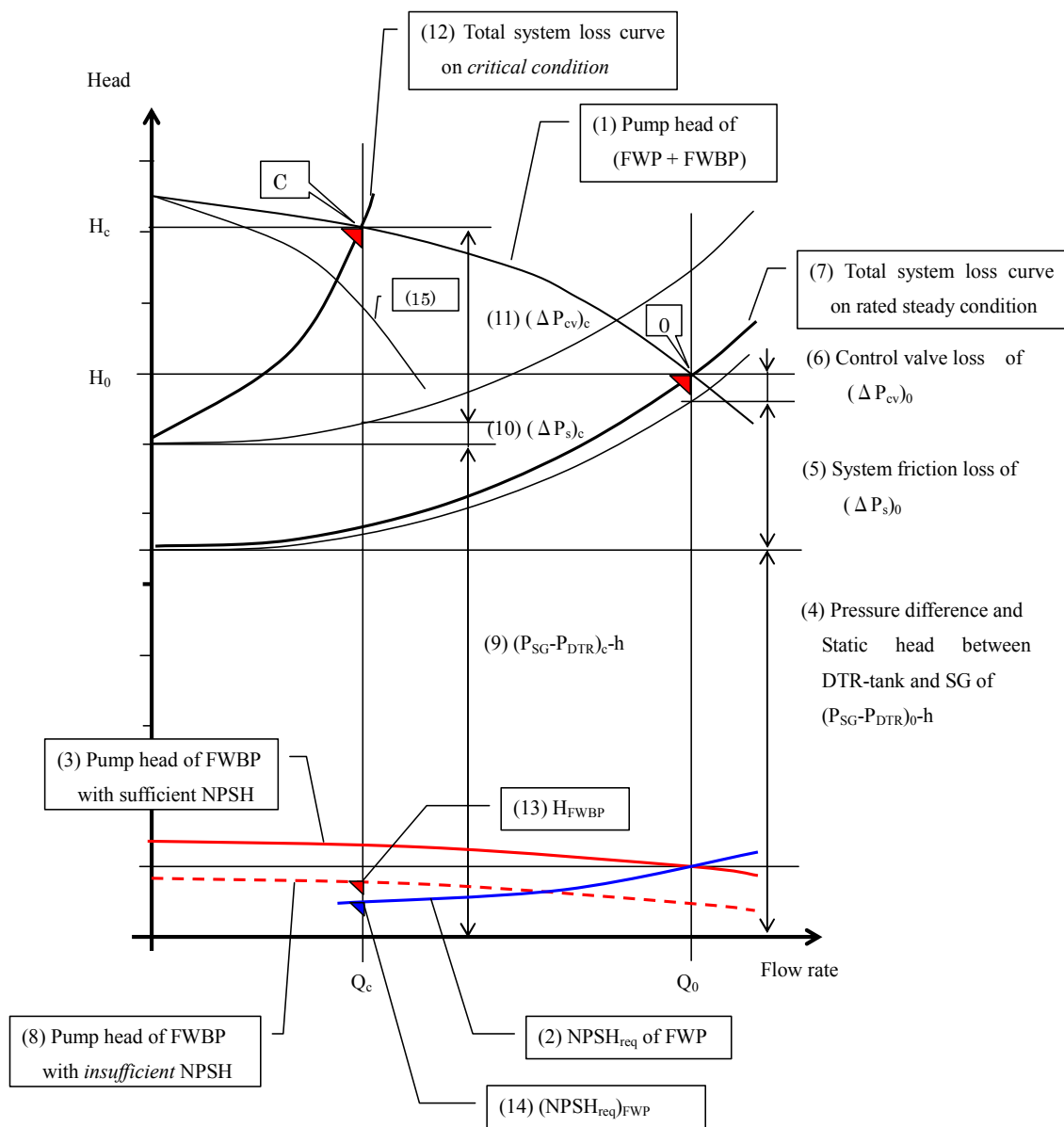
Fig. 4.21 System loss curve and head of FWP
