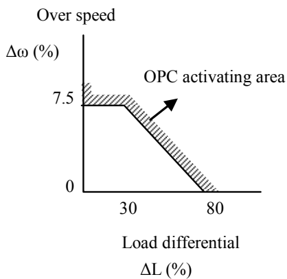
Fig. 1.5 Activation area of OPC system
