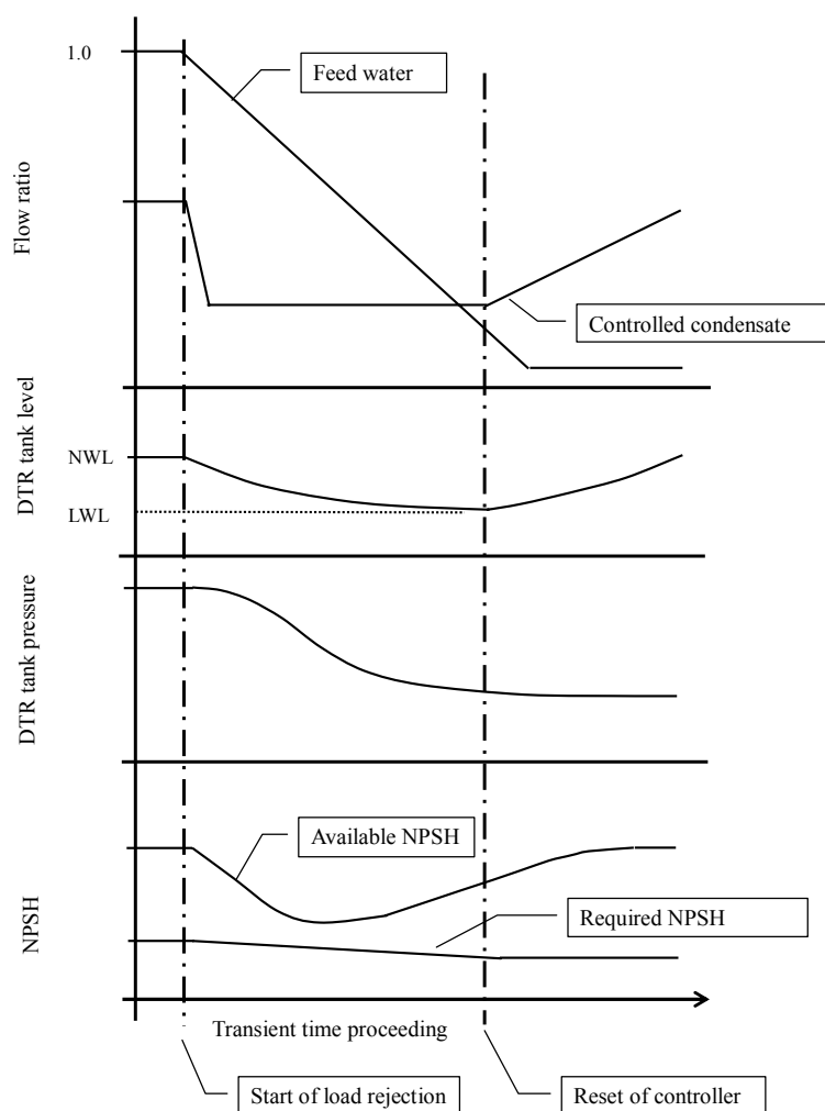
Fig. 4.25 Transient behavior with NPSH controller
