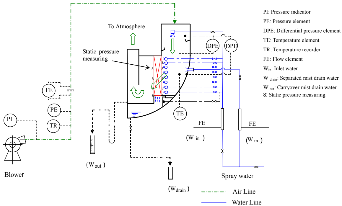
Fig. 2.15 Test facility flow diagram of air-water test
