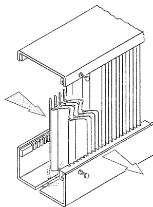
Fig. 2.9 Advanced type mist separator vane
