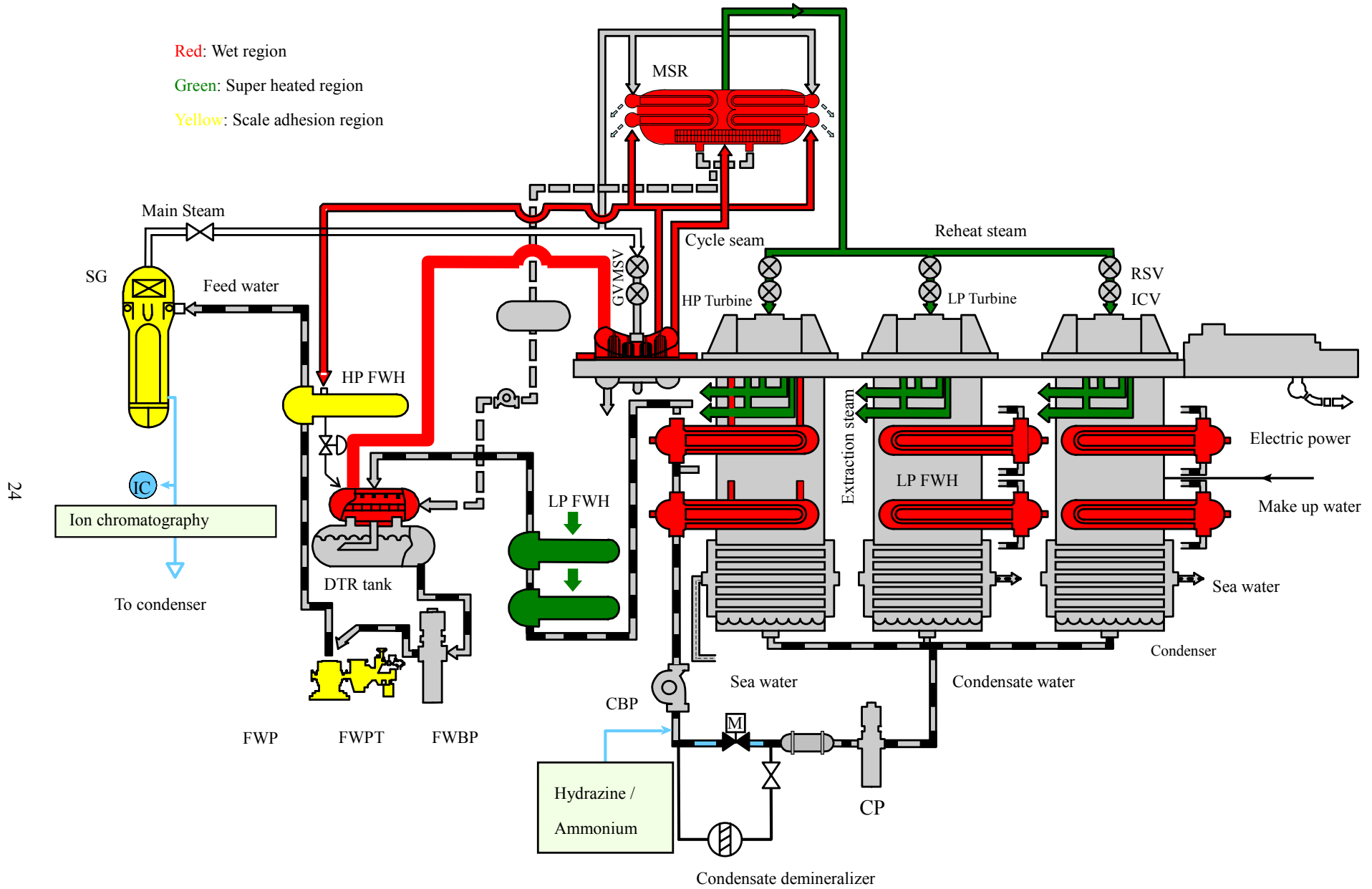
Fig. 1.13 FAC and scale adhesion region of NPP turbine system
