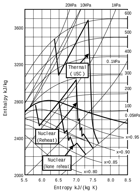
Fig. 1.3 Turbine expansion line both of nuclear and fossil
