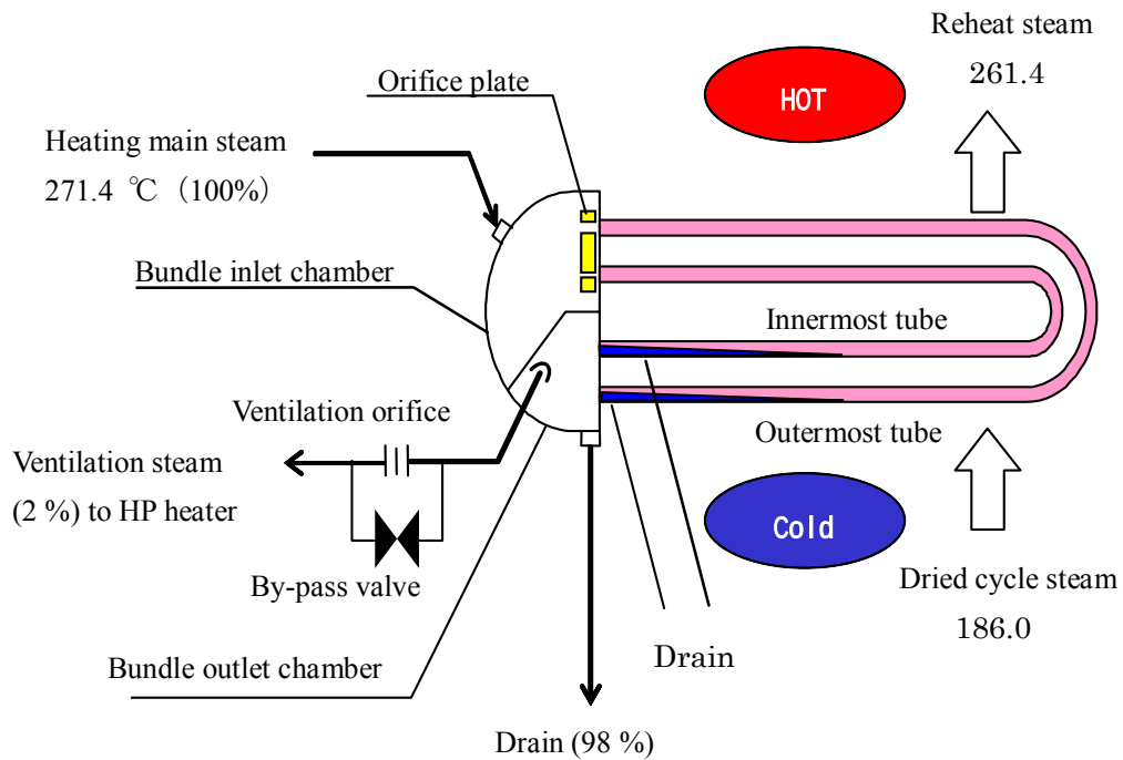
Fig. 1.20 Drainage of MSR heat exchanger tube
