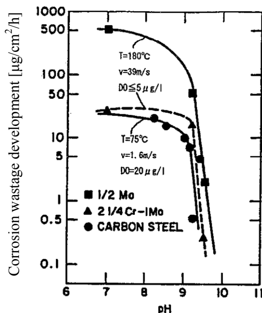
Fig. 3.1 Flow accelerated corrosion developing rate depending on pH for various kinds of materials
