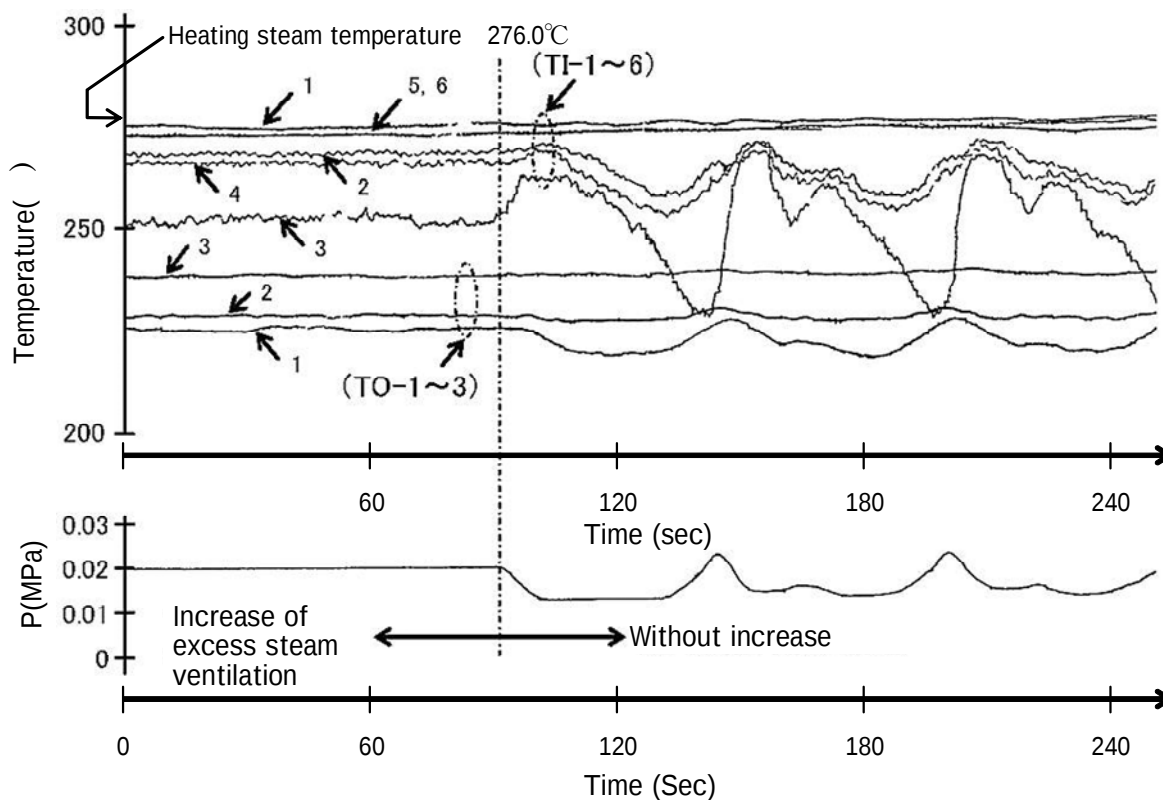
Fig. 2.30 Tube drain instability with and without increase of excess steam ventilation at 50% turbine load
