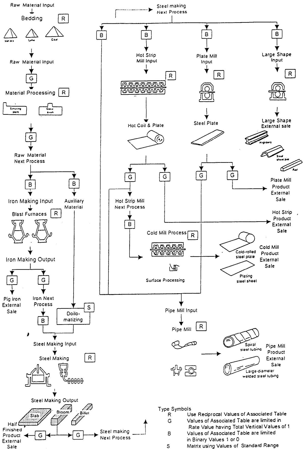
Figure 7-5 Block diagram of Material Flow in Integrated Iron and Steel Works
