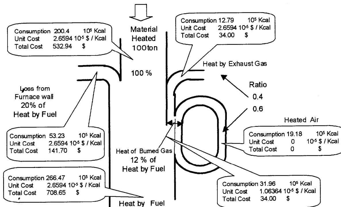
Figure II-61 Calculated Energy Flow and Cost Flows
