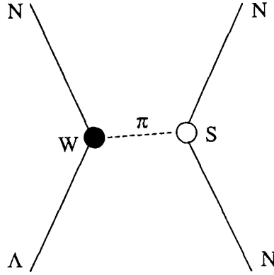
Figure 2.3: One pion exchange diagram.
