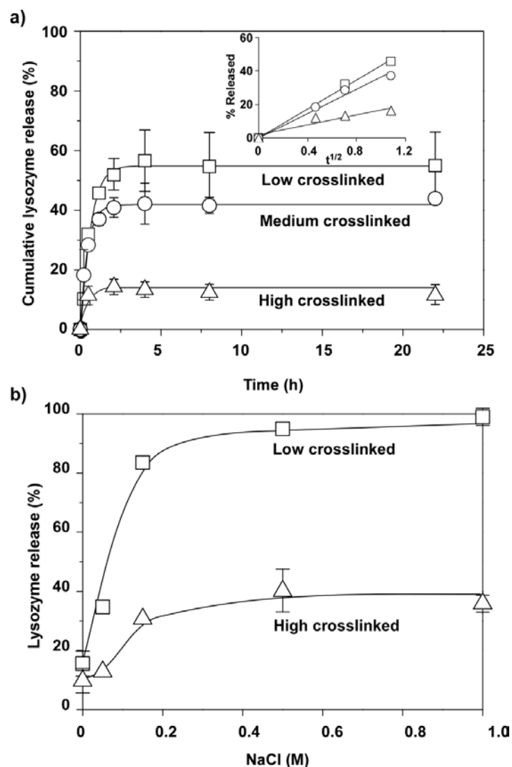
Fig. 3-5. Release of lysozyme from HA-Tyr hydrogels formed with 0.124 U/ml of HRP and (□) 473, (○) 582 and (△) 728 \mu\text{M} of \text{H}_2\text{O}_2 . a) Cumulative release against time, the inset shows cumulative release as a function of the square root of time ( n = 2-3 , mean \pm SD). b) Percentage of lysozyme released when the hydrogels were incubated in various concentrations of NaCl for 4 h ( n = 3 , mean \pm SD).
