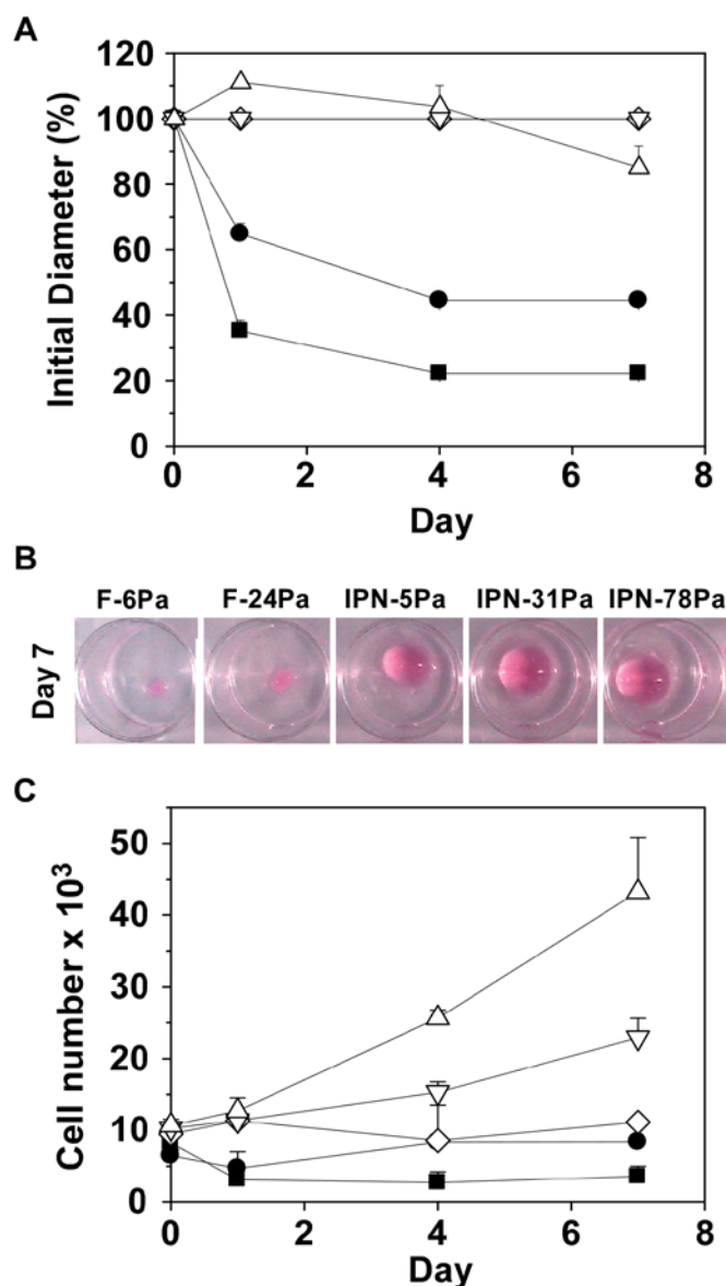
Fig. 5-20. Floating culture of hydrogels containing fibroblasts. (A) Gel contraction by cells expressed as percentages of initial gel diameter for F-6Pa (■), F-24Pa (●), IPN-5Pa (Δ), IPN-31Pa (▽) and IPN-78Pa (◇). (B) Photographs of the gels after culture for 7 days. (C) Corresponding proliferation of fibroblasts as measured by DNA quantification (n = 3).
