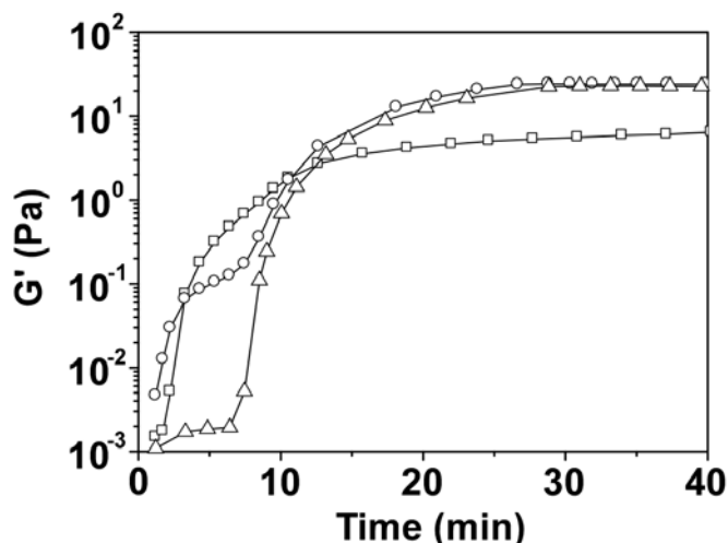
Fig. 5-16. Development of G' of the fibrin gel (2.5 mg/ml) (□), HA-Tyr hydrogel (2.5 mg/ml) (Δ) and fibrin-HA-Tyr IPN hydrogel (2.5 mg/ml each) (○). Both the HA-Tyr hydrogels and IPN hydrogels were formed with 98 \mu\text{M} of \text{H}_2\text{O}_2 . The thrombin and HRP concentrations were 0.31 NIH U/ml and 0.16 U/ml, respectively.
