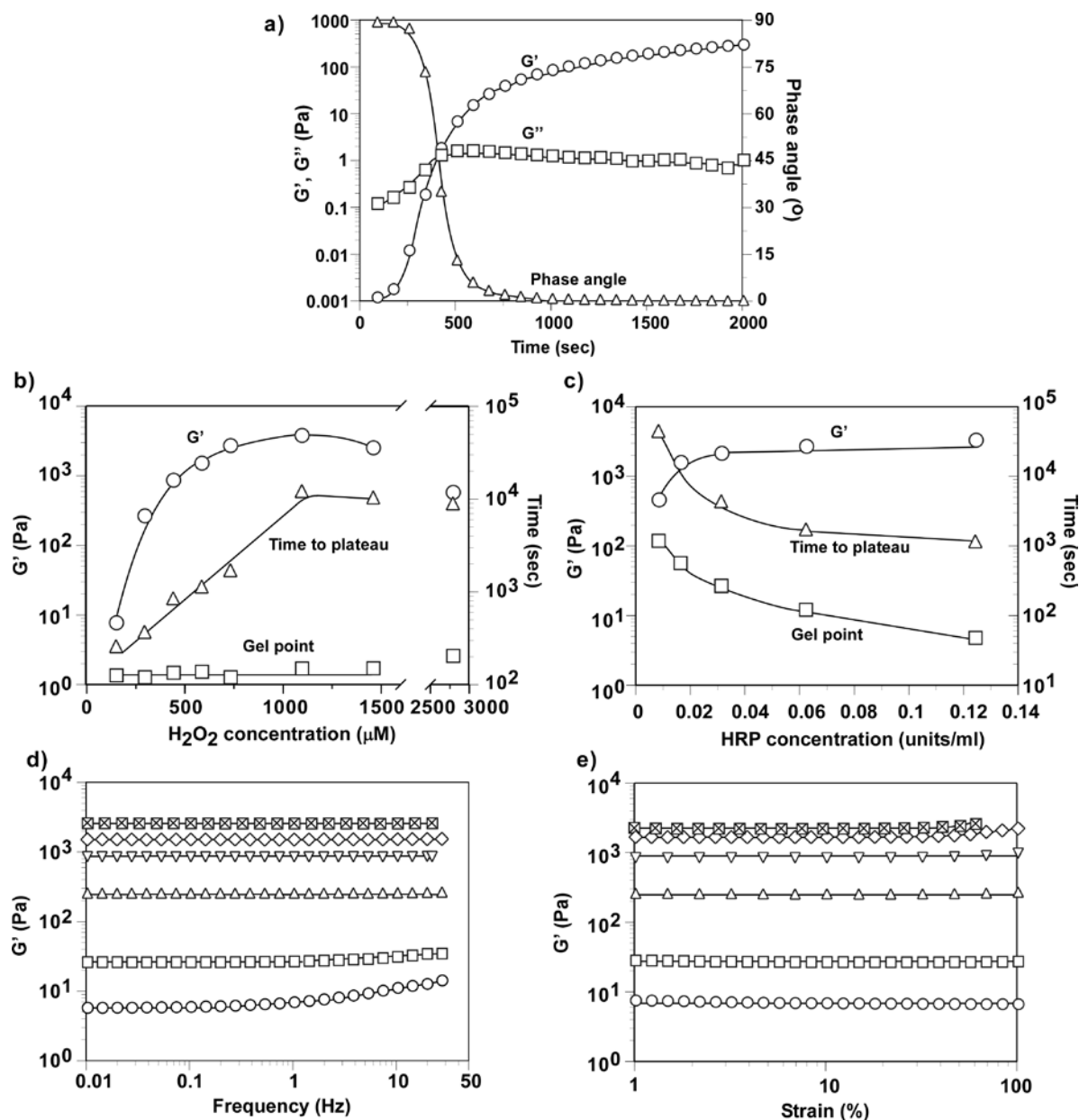
Fig. 2-2. Rheological characterization of HA-Tyr hydrogels. (a) Typical evolutions of the storage modulus G' (○), loss modulus G'' (□) and phase angle \delta (△) of HA-Tyr hydrogel formed with 0.025 U/ml of HRP and 728 \mu\text{M} of \text{H}_2\text{O}_2 . Measurement was taken with a constant deformation of 1% at 1 Hz, 37 °C. Effects of (b) \text{H}_2\text{O}_2 and (c) HRP concentration on the G' (○), the gel point (□) and the time needed for G' to reach plateau (△). HRP and \text{H}_2\text{O}_2 concentrations are fixed to 0.062 U/ml for (b) and 728 \mu\text{M} for (c), respectively. (d) Frequency sweep and (e) amplitude sweep of hydrogels formed with 0.062 U/ml of HRP and 146 (○), 160 (□), 291 (△), 437 (▽), 582 (◇), and 728 (⊠) \mu\text{M} of \text{H}_2\text{O}_2 .
