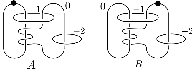
Figure 1.9: Kirby diagrams for A and B .
