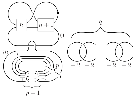
Figure 2.3: Kirby diagram for C_2(m, n, p, q)
