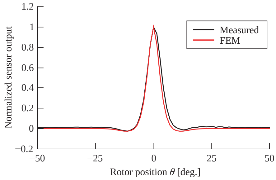
Fig. 3.33: Comparison of calculated and measured point load response functions. Each sensor output is normalized.
