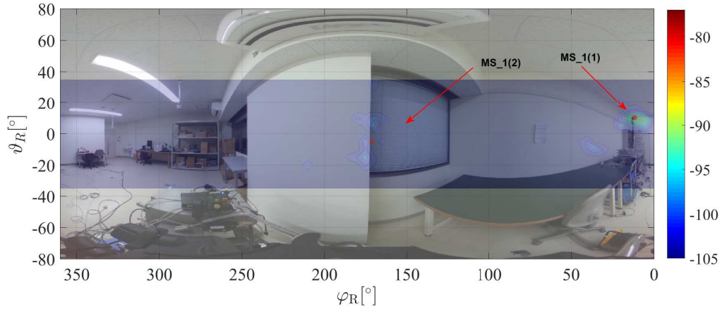
Figure 5-7: The expol APS(\Omega_R) at MS_1
