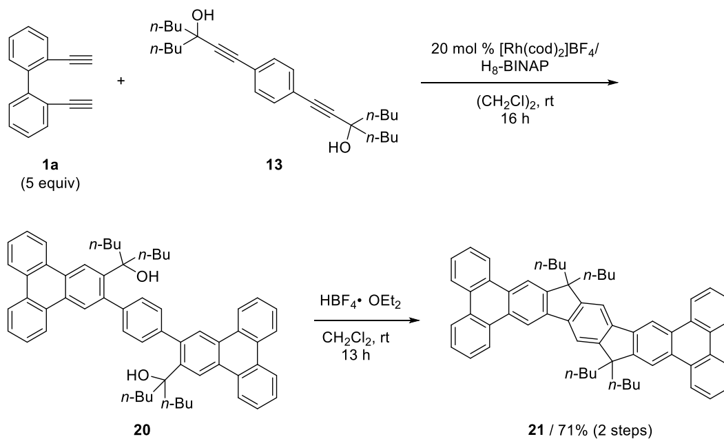
Scheme 1.6. Synthesis of ladder molecule 21 .
