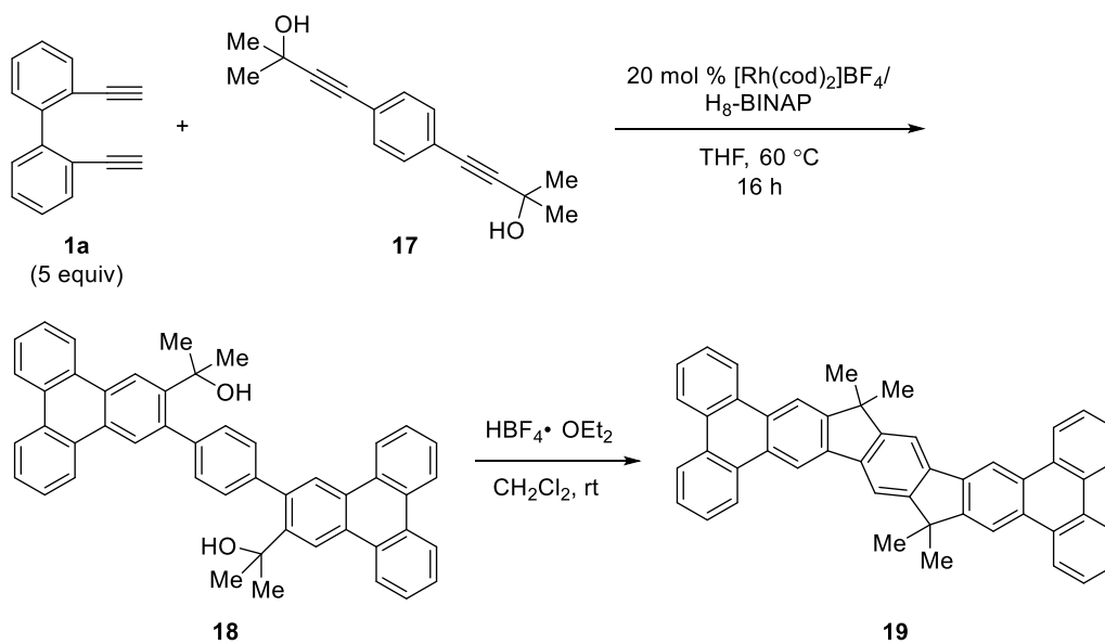
Scheme 1.5. Synthesis of ladder molecule 19 .
