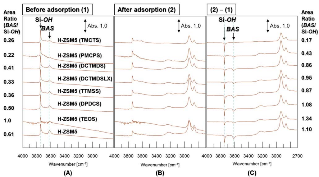
Fig. 4A IR spectra (A) before and (B) after adsorption of hexamethyleneimine to parent and silylated H-ZSM5 and (C) subtracted spectra of (A) from (B)
