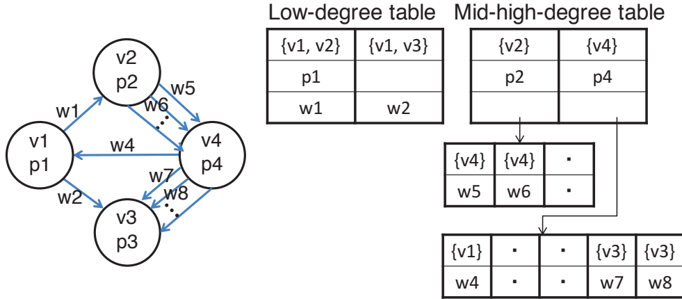
Figure 4.2: Overview of Degree Aware Dynamic Graph Data Structure (DegAwareRHH)
