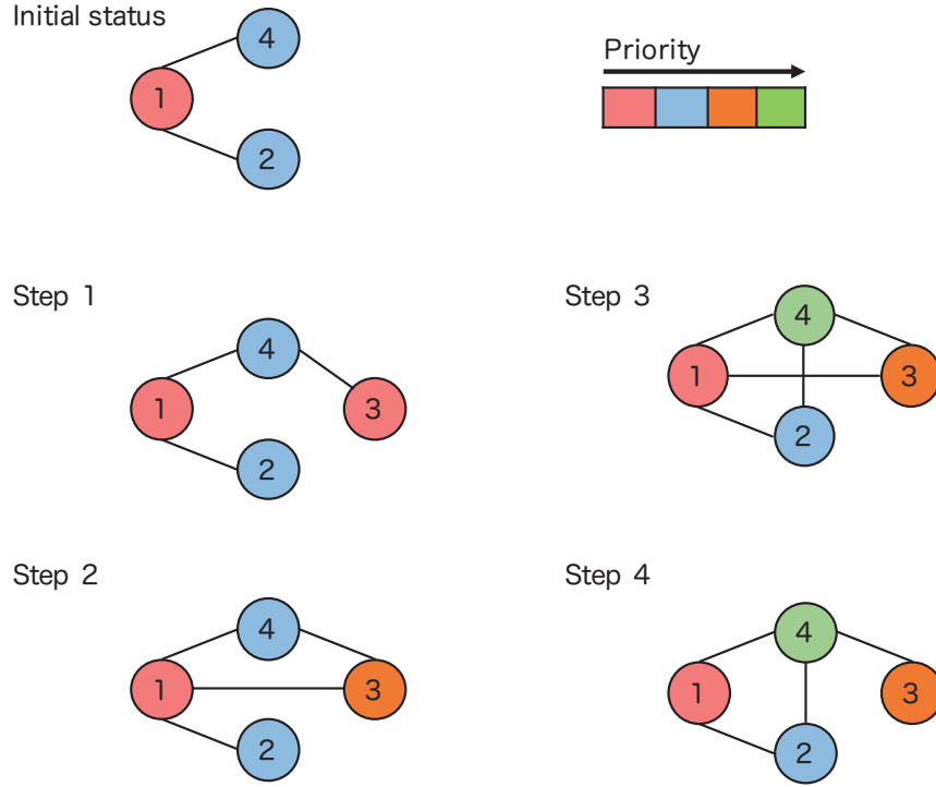
Figure 4.20: An Example of the Dynamic Graph Colouring Algorithm
