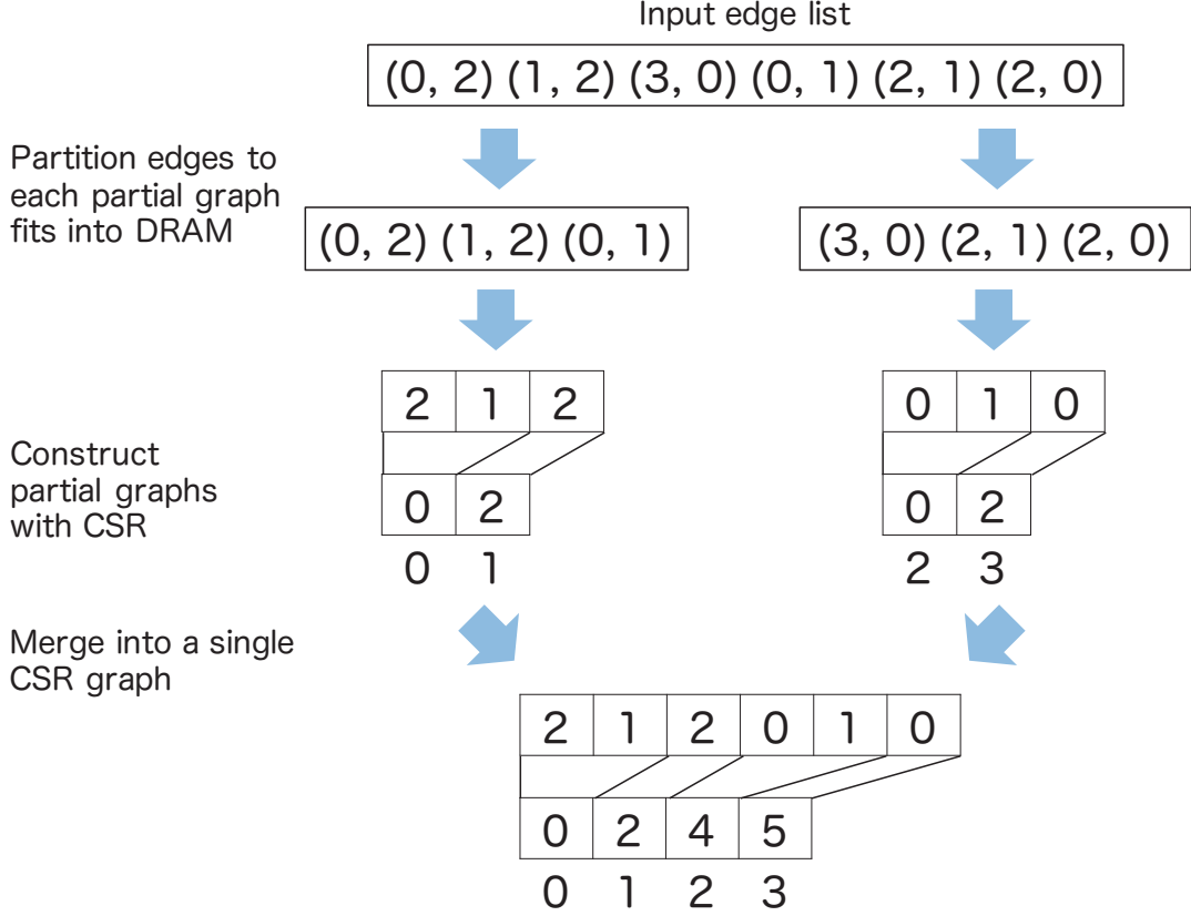
Figure 3.7: Out-of-core Graph Construction
