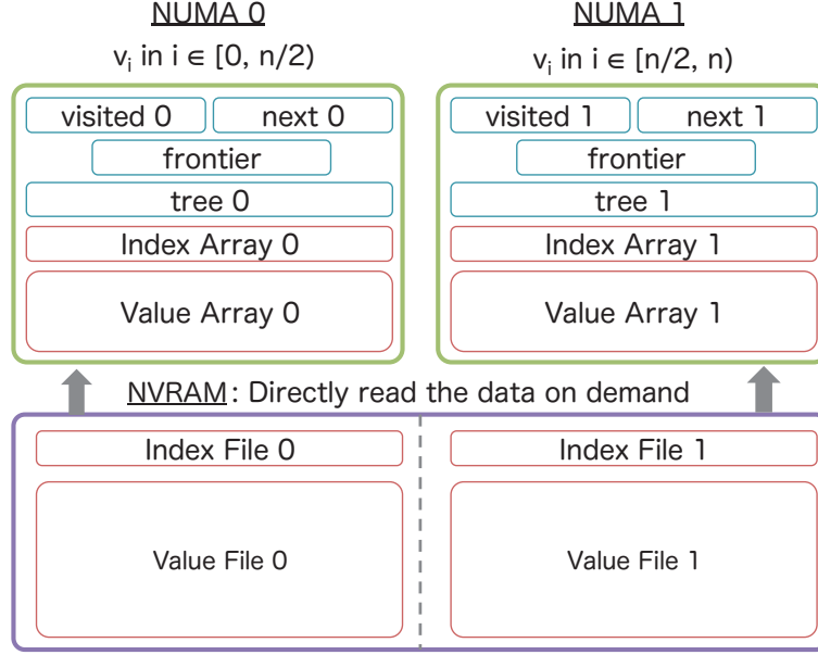
Figure 3.6: Data Structures of Out-of-core Hybrid BFS with Single Graph Model
