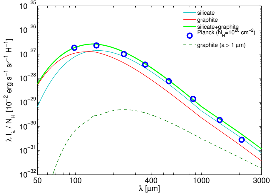
Figure 5.8 Comparison of our model to the observed emission from Planck , in the model (1).
