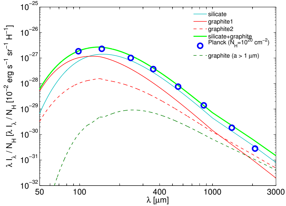
Figure 5.9 Comparison of our model to the observed emission from Planck , in the model (2).
