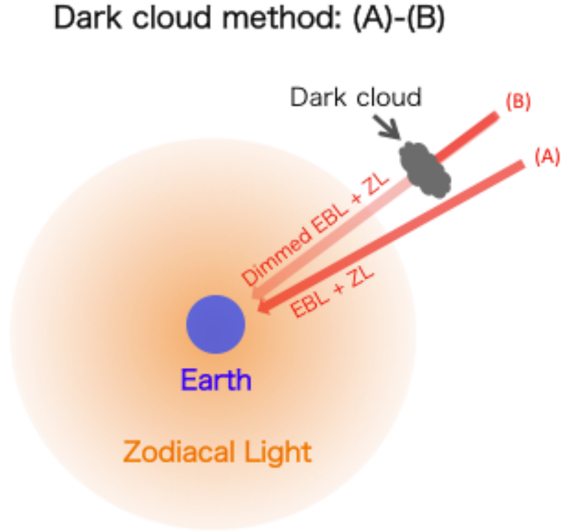
Figure 1.5 Conceptual diagram of EBL measurement using dark cloud method.
