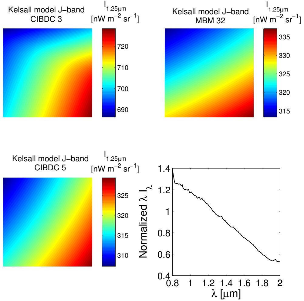
Figure 3.6 The ZL gradient at 1.25 \mu\text{m} for each field based on the model of Kelsall et al. (1998) and the spectrum of ZL derived by Arai et al. (2015). The top left panel is the ZL gradient in CIBDC 3 field, the top right panel is MBM 32's, the bottom left panel is CIBDC 5's, and the bottom right panel indicates the spectrum of ZL normalized by 1.25 \mu\text{m} .
