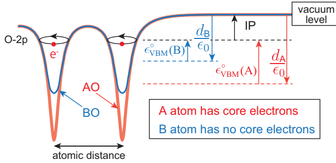
FIG. 5. Schematic of the relationship between electrostatic potential (solid lines), macroscopic dipole potential energy d/\epsilon_0 , and bulk electronic eigenvalues \epsilon_{\text{VBM}}^{\circ} of hypothetical oxides AO and BO. We assume that these two oxides have the same crystal structures and same IPs (see text for details). Although the IPs are the same, d/\epsilon_0 and \epsilon_{\text{VBM}}^{\circ} are very different, which is attributed to the core electrons in A atoms.
