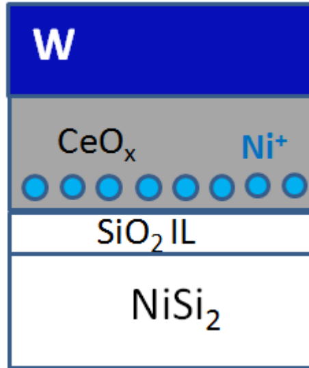
Figure 5.7. Fresh sample illustration for W/CeO x /SiO 2 /NiSi 2 structure ReRAM
