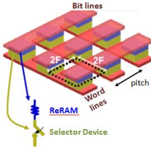
Figure 1.12 Structure of ReRAM and its selector device in memory matrices [1.1]
