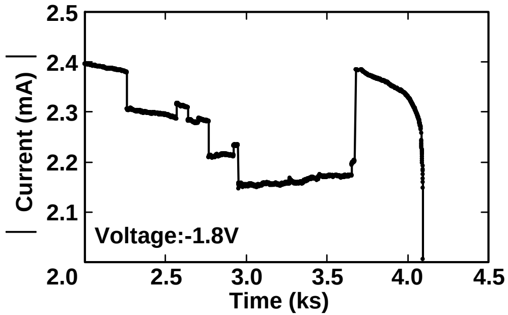
Figure 6.4 Extended figure of time dependence when reset voltage set -1.8V
