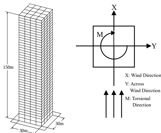
Fig.2 Wind Direction and Structural Axes
