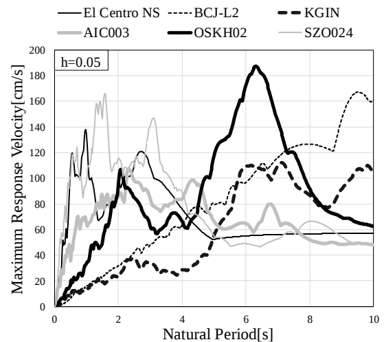
Fig.5 Seismic Response Spectra
