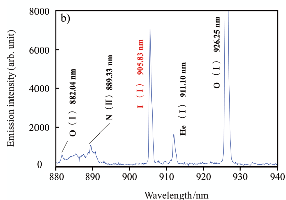
Fig. 8 Emission spectra of (a) \text{CH}_2\text{Br}_2 and (b) \text{C}_2\text{H}_5\text{I} .
