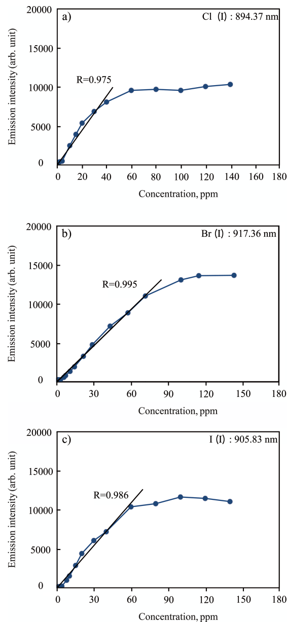
Fig. 9 Calibration curves for (a) chlorine, (b) bromine, and (c) iodine.
