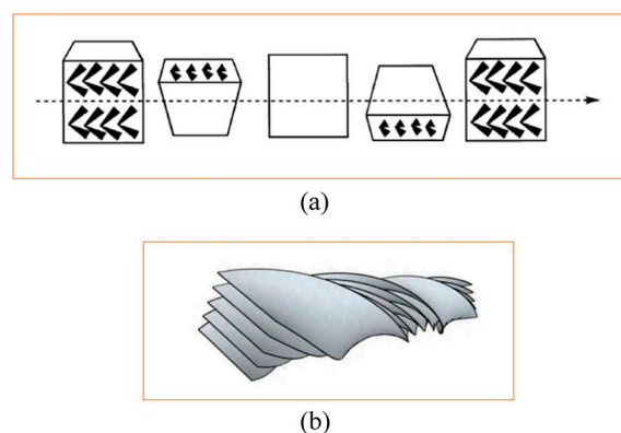
Fig. 6 (a) TGB-like helical structure and (b) nano-filament helical structure proposed for B4.
