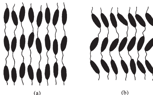
Fig. 1 Layered structures of smectic phases of (a) BB-n (even) and (b) BB-n (odd).
