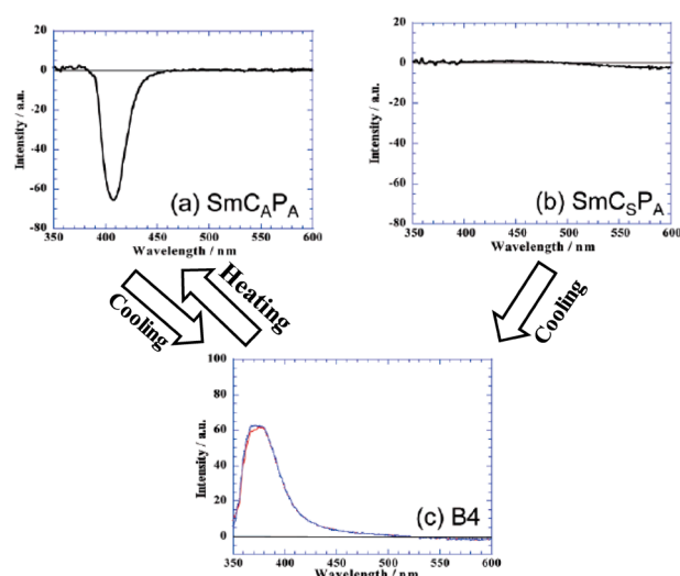
Fig. 8 CD spectra observed in P-12-O-PIMB containing 10 wt% of chiral P-8-O-PIMB6*: (a) homochiral \text{SmC}_A\text{P}_A and (b) racemic \text{SmC}_S\text{P}_A of B2 phase, and (c) B4 phase. Homochiral \text{SmC}_A\text{P}_A shows the clear negative CD peak while racemic \text{SmC}_S\text{P}_A no CD peak. When the racemic \text{SmC}_S\text{P}_A was initially prepared from isotropic melt and then cooled to the B4 phase, the positive CD peak appeared around 380 nm as in (c). On heating back to the B2 zone, the strong negative CD peak characteristic of the homochiral \text{SmC}_A\text{P}_A structure is detected. Hereafter, the spectra (a) and (c) are altered upon temperature cycling between B2 and B4.
