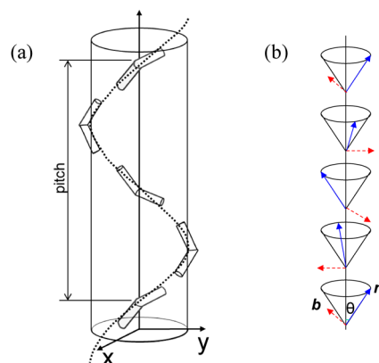
Fig. 10 (a) Spontaneously modulated nematic phase for K_3 < 0 : conical twist-bend helix with twofold degenerated twist (left or right) and (b) its conical local director distributions of \mathbf{n} - and bend \mathbf{b} -directors. Here \mathbf{n} rotates along the z -axis on a revolution cone with aperture \theta , enabling the local bend \mathbf{b}(z) to remain always at its spontaneous value |\mathbf{b}(z)| = |\mathbf{b}_s| . In achiral systems this bend-twist texture is twofold degenerated, with both right-hand and left-hand twist permitted. The twist is not spontaneous, but imposed by the bend, enabling a kind of a “third dimension escape” of \mathbf{n} from the geometrical constraints.
