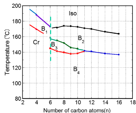
Fig. 3 Phase transition behavior in P-n-O-PIMB with n=4, 6-12, 14, 16 .
