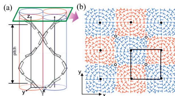
Fig. 12 Schematic illustrations of a) a twist-bend director distribution alike N_{TB} phase forming right-handed (blue) and left-handed (red) helical ordering and b) a possible image of molecular projection (shown by nail) and skyrmion-type 2D tetragonal lattice model based on cylindrical arrays by neighboring opposite helicity. The nails indicate the b -directors shown in Fig. 10.
