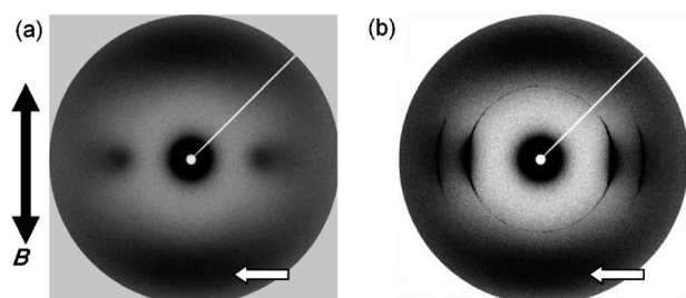
Fig. 11 Oriented 2D SAXS profiles of a) N1 and b) N2 phases. “B” is the magnetic field direction.
