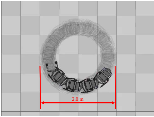
Fig. 10. Turning Simulation with a Vrep simulator. Only yaw joints are bent.
