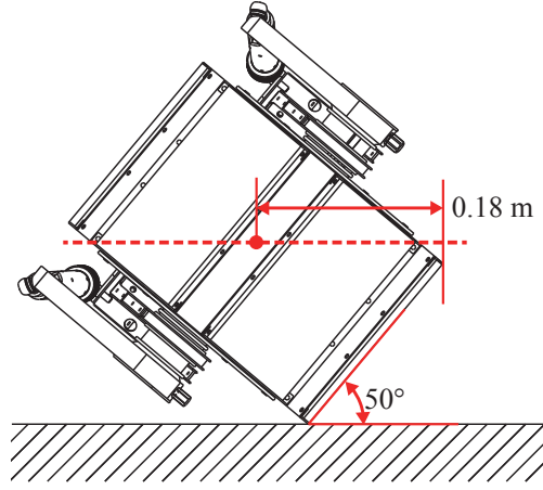
Fig. 9. Turning motion.
