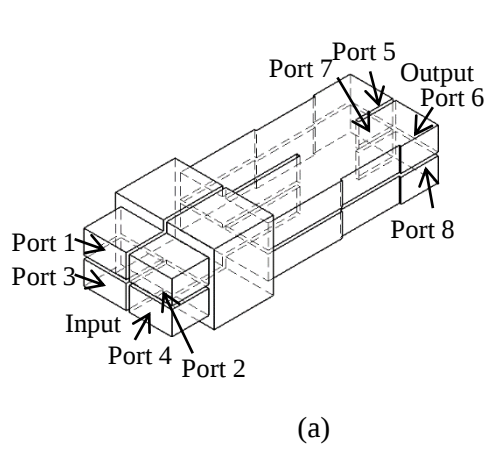
Fig. 2.7 4×4-way short-slot combined coupler (a) Horizontally stacked short-slot E-plane coupler (b) Vertically stacked short-slot H-plane coupler (c) Combination of (a) and (b)
