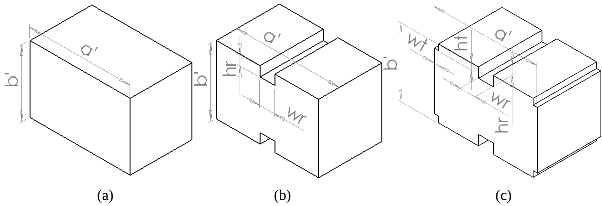
Fig. 2.11 The coupled region (a) Rectangular waveguide (b) Double ridge rectangular waveguide (c) Trim the outermost vertices of double ridge rectangular waveguide.
