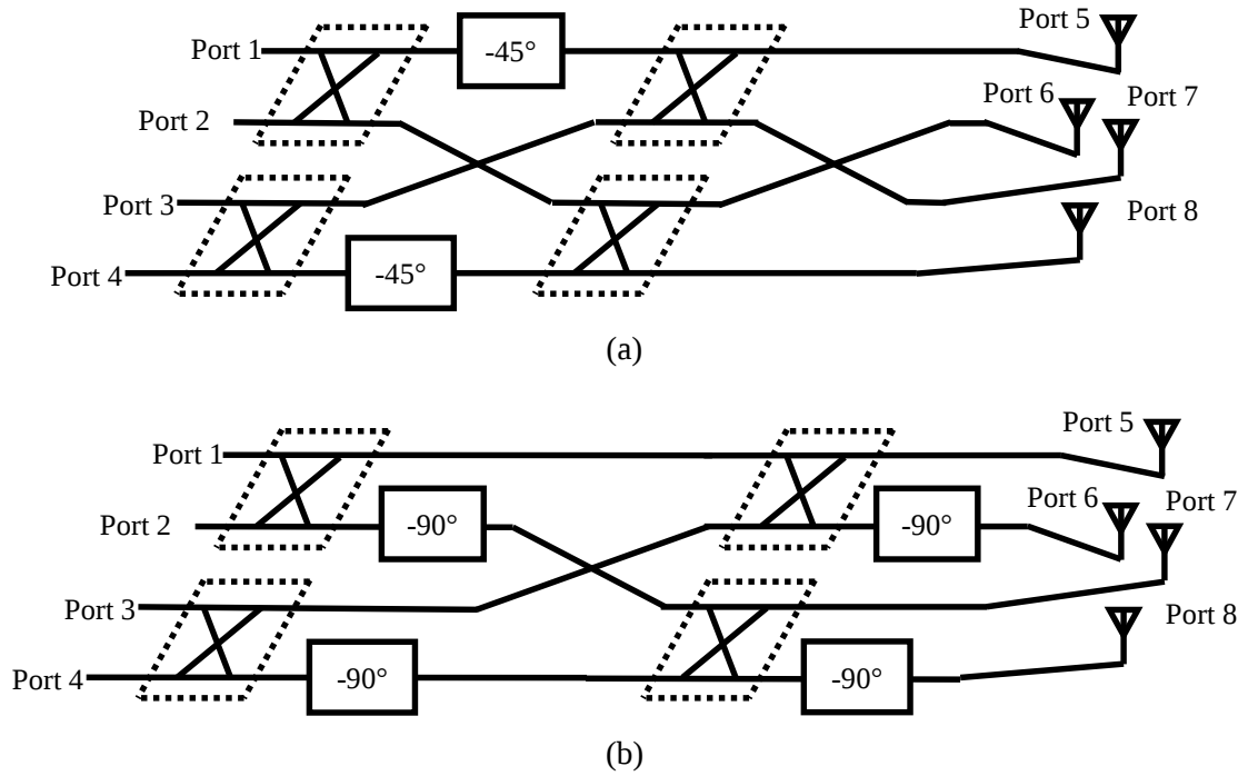
Fig. 2.6 2×2 array antenna fed by 4×4-way 1-D beam-switching Butler matrix (a) Original (b) Modified.
