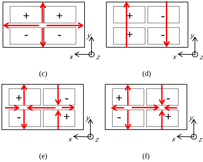
Fig. 2.10 Electric field distribution and its polarities in the coupled region (a) TE 10 (b) TE 11 (c) TM 11 (d) TE 20 (e) TE 21 (f) TM 21 . Solid black lines: Boundary of the coupled regions, Dotted black lines: Boundary of the port branches.
