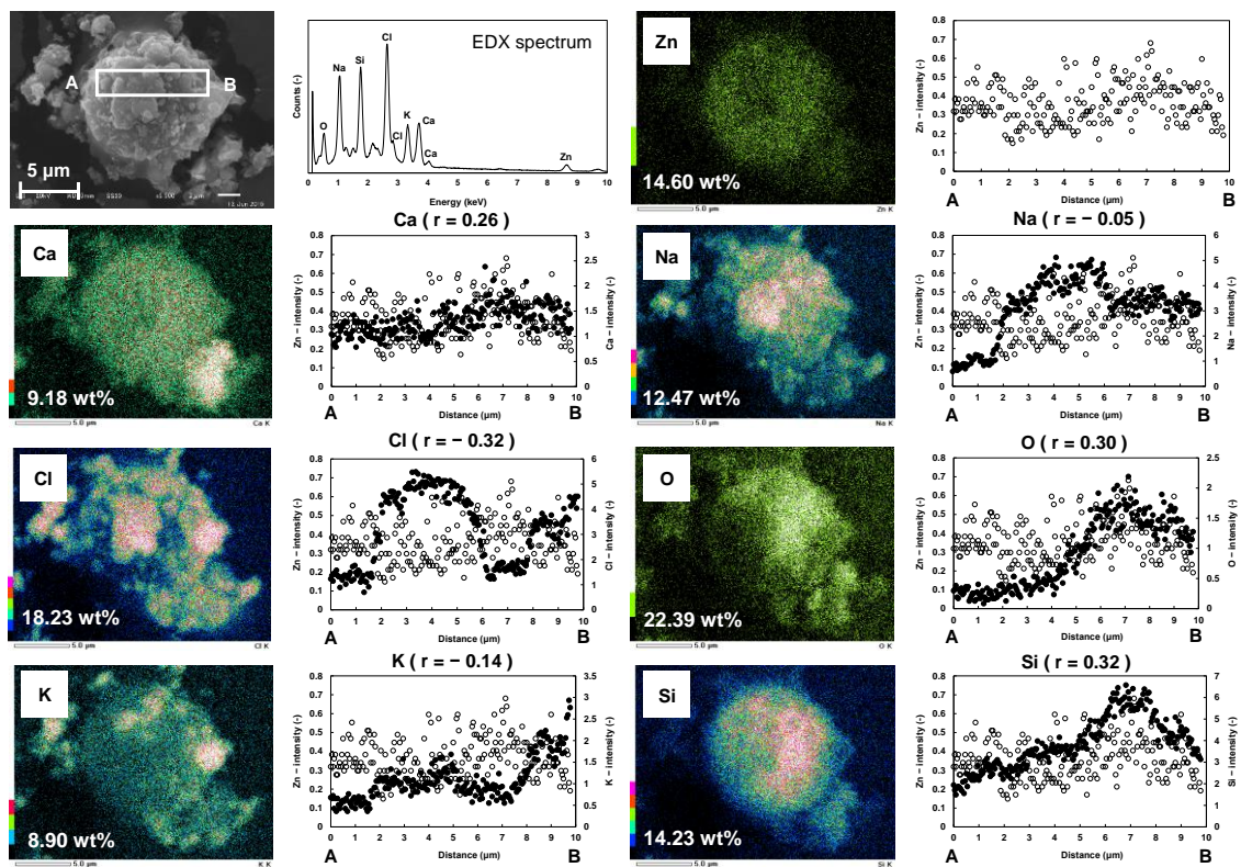
Fig. A.3 Elemental distributions and micro-scale correlation analysis along point A to point B on Zn-rich particle (ZnO or Zn 2 SiO 4 ) in raw MSWI fly ash ( r : correlation coefficient)
