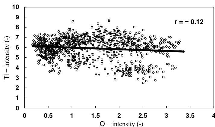
Fig. 5.5 Scatter plot for intensity data of O and Ti (r : correlation coefficient)
