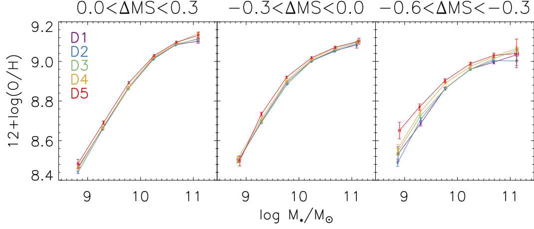
Figure A.1: Mass–metallicity relation for the three \Delta\text{MS} subsamples. For each panel, we further split the sample into five environmental bins (D1–D5) as indicated in the left panel.
