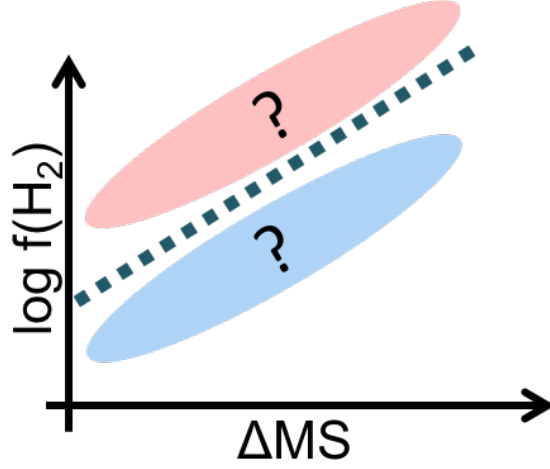
Figure 1.4: Schematic view of the correlation between \Delta MS and f_{H_2} . Dotted line indicates the correlation in general (field) environment.
