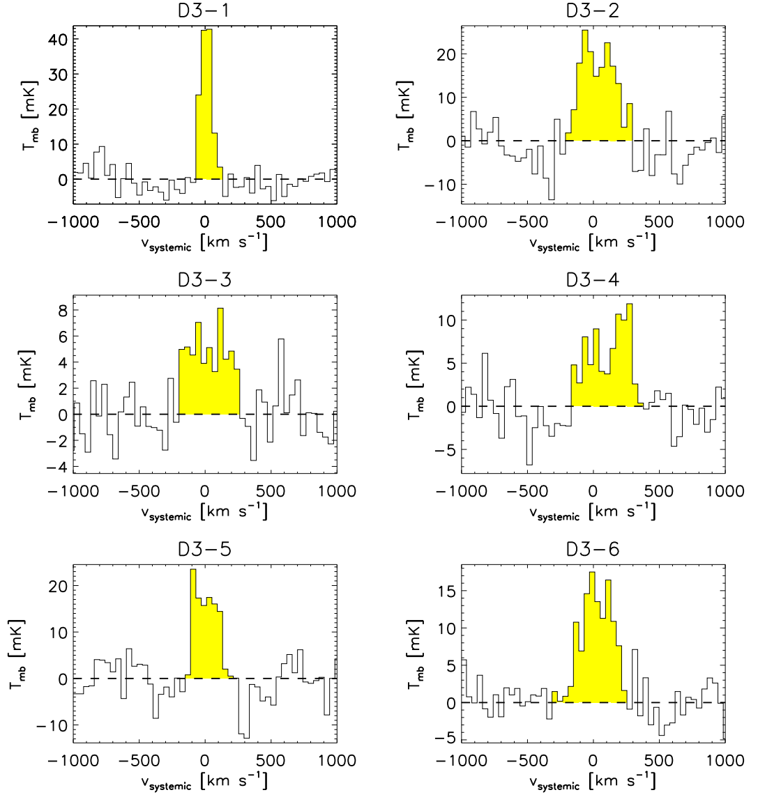
Figure 2.6: The CO spectra of D3 galaxies.
