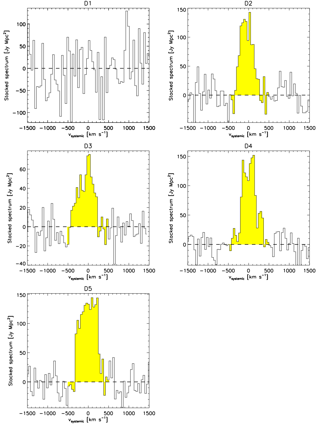
Figure 3.5: The stacked CO spectra for COLDGASS sample with \Delta MS < -1 for each environmental bin.
