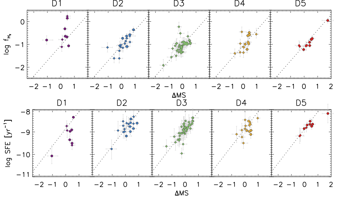
Figure 3.8: Same plots as Figure 3.2 and 3.3 in the case we apply the non-universal \alpha_{\text{CO}} (see Eq. 3.6).
