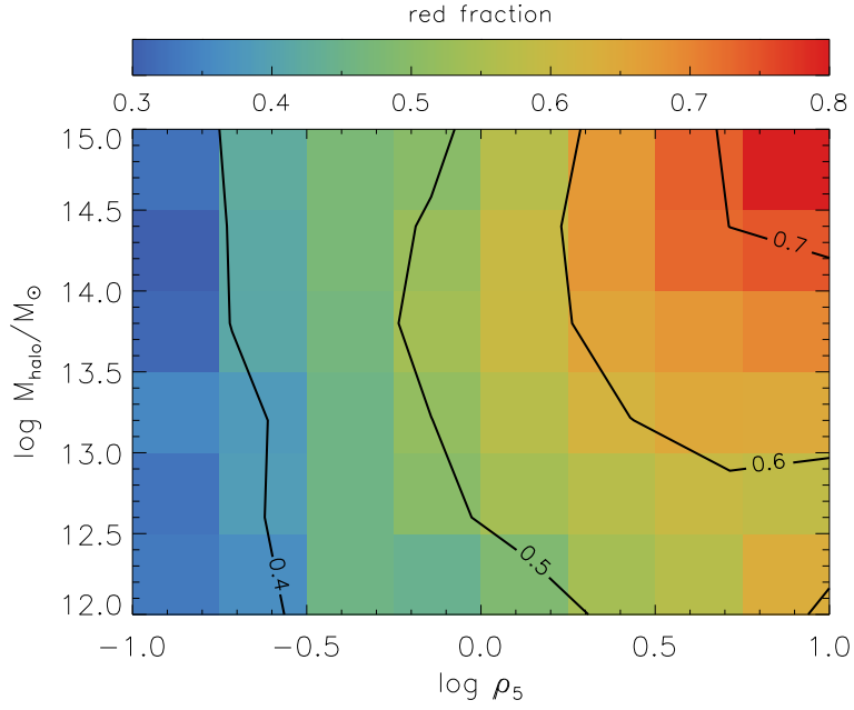
Figure 3.10: The distribution of red fraction(= N(\Delta_{\text{MS}} < -1)/N(\text{total}) ) on \rho_5 - M_h plane.
