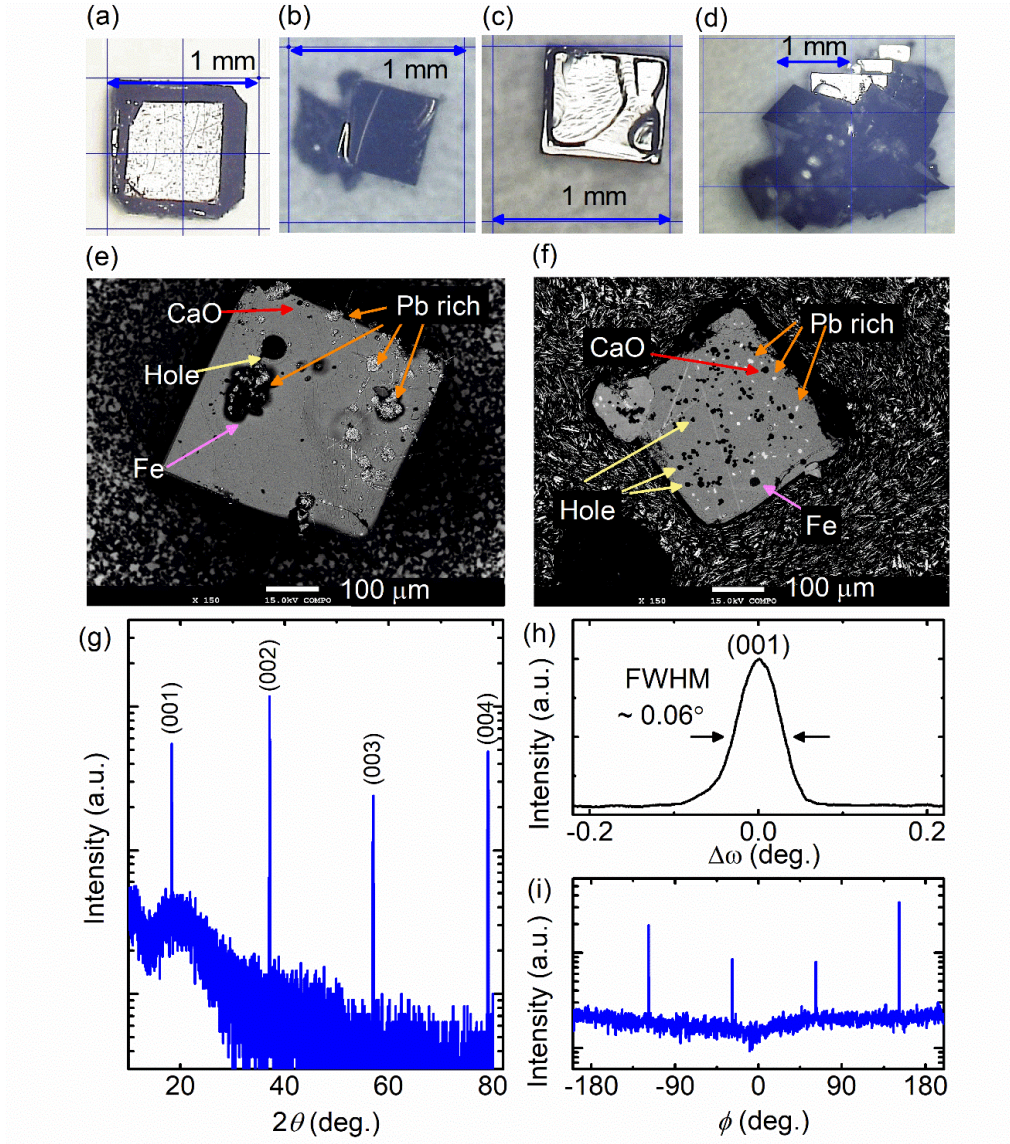
Figure 3.3: Characterization of the samples grown in different crucibles. (a)-(d) Microscope images of crystals grown in stainless steel (a), Mo (b), and Fe crucibles (c, d), respectively. (e),(f) Compositional images of the crystals grown in an Fe crucible with filled space before and after the mechanical treatment with sandpaper, obtained by EPMA. Black spots (pointed by red arrows) indicate CaO particles, whereas white spots (pointed by orange arrows) represent surface Pb-rich regions of the \text{Ca}_3\text{PbO} phase. Black spots pointed by pink and yellow arrows show Fe particles and holes, respectively. (g-i) X-ray diffraction (XRD) patterns of a crystal grown in an Fe crucible with filled space. (g) XRD pattern of \theta - 2\theta scan. The observed peaks correspond to the (001) reflections of \text{Ca}_3\text{PbO} , which confirm that the grown crystal was single phase. (h) Normalized rocking curve for the (001) reflection. (i) XRD pattern of \phi scan for the (111) reflection.
