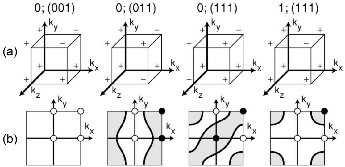
Figure 1.7: Examples illustrating several phases corresponding to \nu_0; (\nu_1, \nu_2, \nu_3) . (a) The signs of \delta_i at the \Gamma_i points on the vertices of a cube. (b) The Fermi surface on a (001) plane for each phase. The product of \delta_i on the projected planes with open (solid) circles illustrating \prod_{i=1}^4 \delta_i = +1(-1) . Between the open and solid circles, there exist odd numbers of Fermi surfaces. On the other hand, even numbers of Fermi surfaces including 0 between open-open or solid-solid circles. In the right most panel, the odd numbers of Dirac cones exit in any crystal planes. In contrast, the surface states do not appear in the left three panels for some crystal planes. These three panels represent WTIs, where the 2D TIs are aligned along [001] , [01-1] , [11-1] axis respectively and do not have surface states on the planes normal to these axes. The figures are adopted from Ref. [36].
