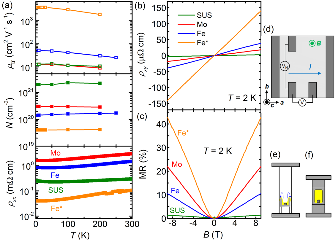
Figure 3.4: Transport properties of crystals grown in stainless steel, Mo, and Fe crucibles. In particular, the data of the crystals grown in Fe crucibles with and without empty space in the stainless steel capsules are illustrated by blue and orange symbols, respectively. (a) Temperature dependence of resistivity \rho_{xx} , carrier density N , and transport mobility \mu_{tr} . (b),(c) Field dependence of Hall resistivity \rho_{xy} and magnetoresistance (MR) at 2 K. (d) Schematic of the four-probe configuration for the transport measurements in which the current flows along the a axis on the ab plane with the magnetic field applied along the c axis. (e),(f) Schematic images of stainless steel capsules with and without empty space, respectively. Yellow parts and gray cubes represent Ca melt and \text{Ca}_3\text{PbO} crystals formed during the growth process.
