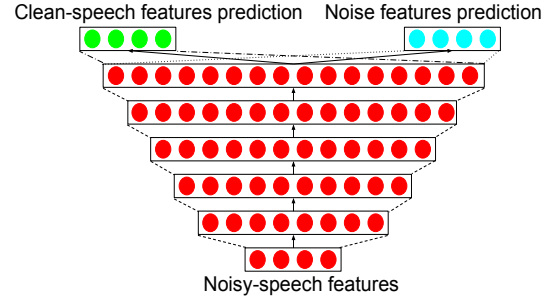
Fig. 4. Structure 2: The same number of nodes with MTAE, but fully connected between layers.
