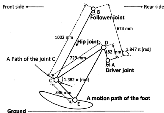
Fig. 4 The designed mechanism
