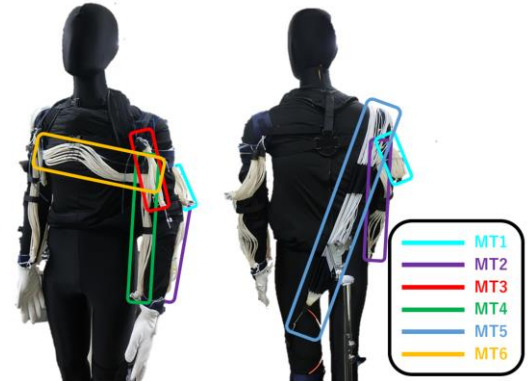
Figure 7. Front view (left) and back view (right) of the soft suit.
