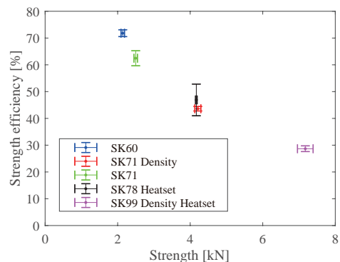
Fig.3 Relationships between strength and bending durability
