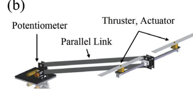
Fig. 7. 1 D.O.F. principle confirmation model: (a) kinematic configuration and (b) 3DCAD model.
