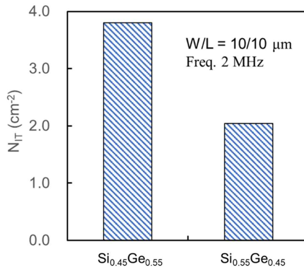
Figure 3-11 Interface trap density ( N_{it} ) for \text{Si}_{0.55}\text{Ge}_{0.45} and \text{Si}_{0.45}\text{Ge}_{0.55} channel pFET with spike RTA temperature 950°C. N_{it} was measured by charge pumping method, frequency of gate bias is 2 MHz.
