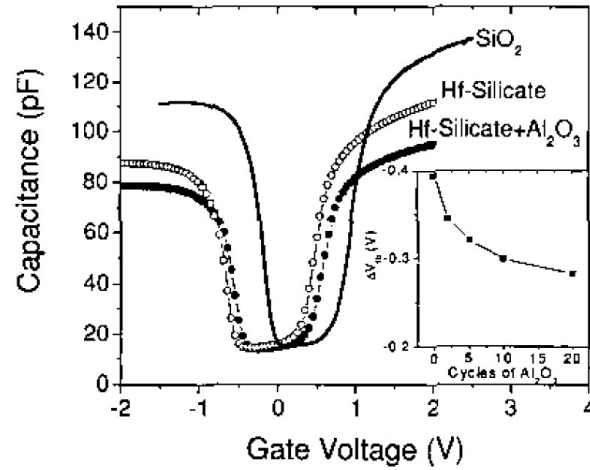
Figure 1-13 C-V characteristics for Poly-Si/(Al 2 O 3 )/HfSiO x stack showing pFET V_T reduction with Al 2 O 3 [27].
