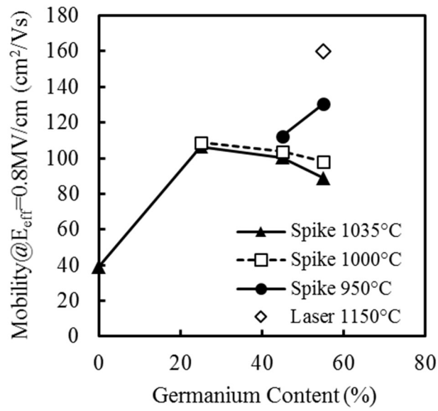
Figure 3-10 High field inversion layer hole mobility (at effective field of 0.8 MV/cm) as a function of Ge content in \text{Si}_{1-x}\text{Ge}_x channel with various activation annealing method / temperature.
