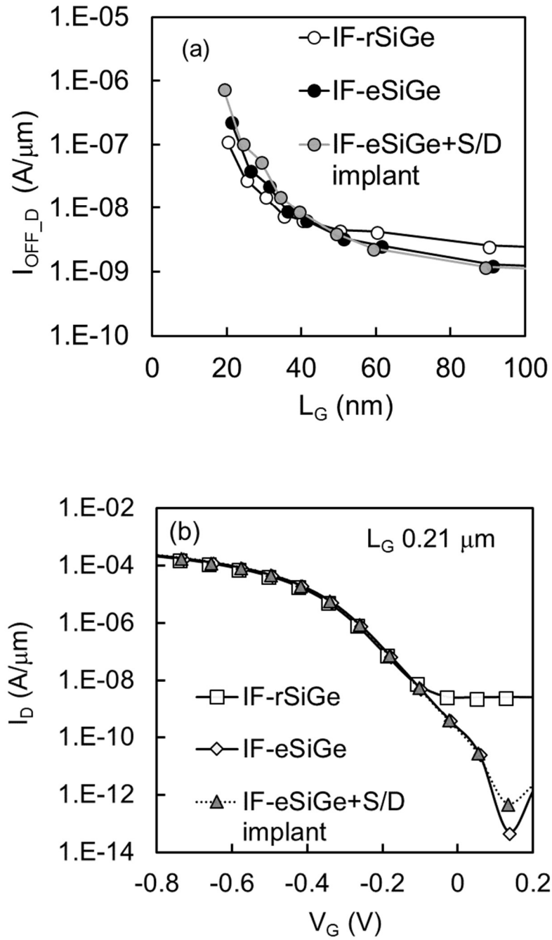
Figure 5-6 (a) I_{\text{OFF\_D}} as a function of gate length for IF-rSiGe and IF-eSiGe devices (w/ and w/o S/D implant). (b) I_D - V_G curve for same devices at L_G = 0.21 \mu\text{m} .
