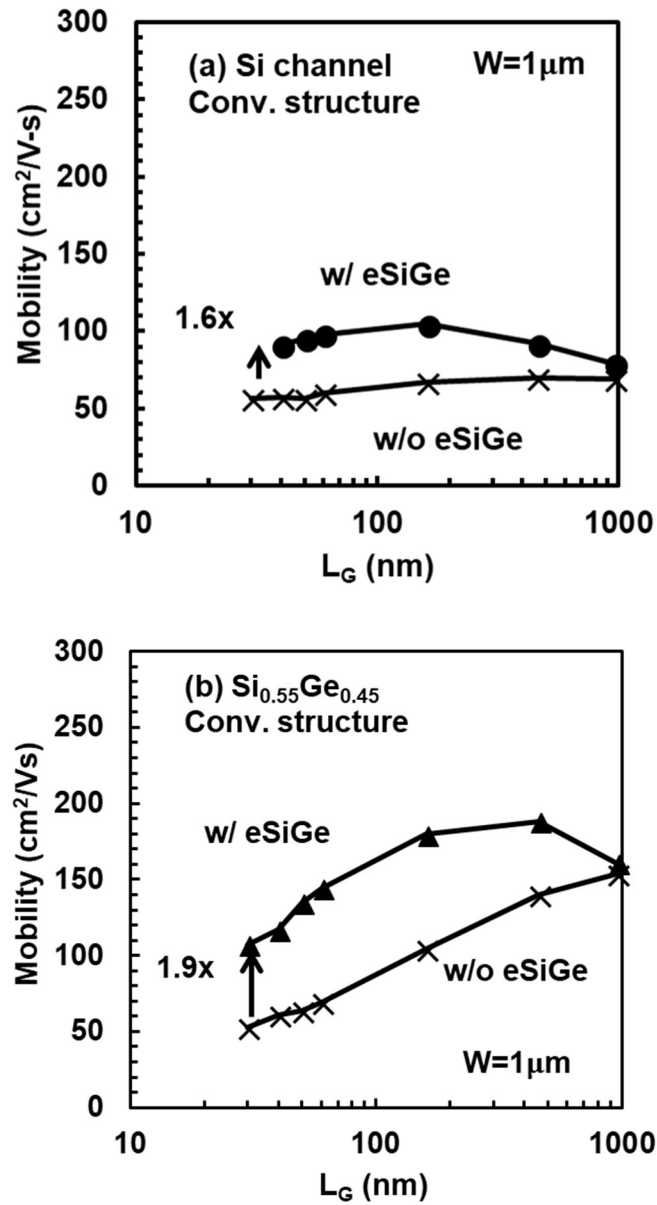
Figure 4-2 Hole mobility as a function of gate length (L G ) for (a) Si channel and (b) Si 0.55 Ge 0.45 channel pFETs. Both are conventional structures (implanted extension and source/drain). eSiGe gives larger or at least comparable hole mobility boost for Si 0.55 Ge 0.45 channel pFET compared to Si channel pFET.
