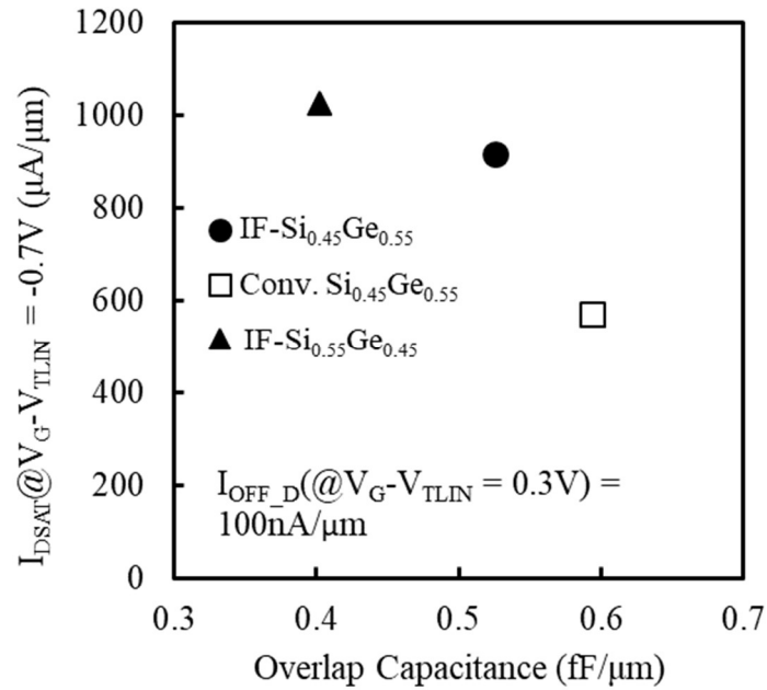
Figure 5-2 I_{\text{DSAT}} ( V_{\text{G}} - V_{\text{TLIN}} = -0.7\text{ V} ) as a function of overlap capacitance. I_{\text{DSAT}} is taken at I_{\text{OFF\_D}} ( V_{\text{G}} - V_{\text{TLIN}} = 0.3\text{ V} ) is 100 nA/ \mu\text{m} . Device channel width is 1 \mu\text{m} for all devices.
