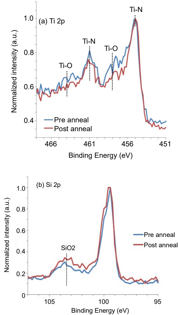
Figure 2-9 AR-XPS results (a) Ti 2p and (b) Si 2pspectra. Pre and post WSA (T 2 ) are plotted.
