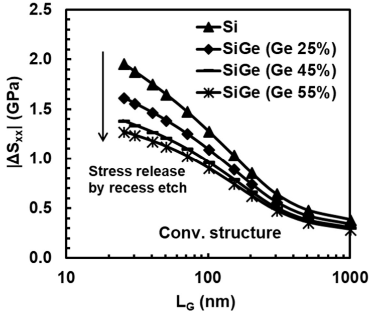
Figure 4-5 Simulated net changes in longitudinal stress ( \Delta S_{xx} ) with eSiGe (stress difference between pre cavity RIE and post eSiGe growth) as a function of gate length for Si and \text{Si}_{1-x}\text{Ge}_x channel with various Ge content. The net stress gain ( \Delta S_{xx} ) monotonously decreases as Ge content in \text{Si}_{1-x}\text{Ge}_x channel increases. This is because \text{Si}_{1-x}\text{Ge}_x channel with higher Ge content loses higher amount of strain during cavity RIE.
