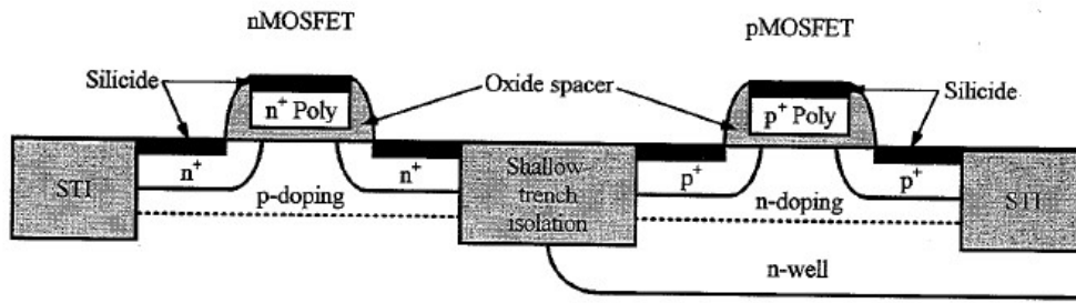
Figure 1-2 A schematic cross section for modern CMOS transistors [3].
