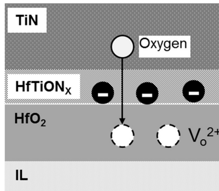
Figure 2-12 Schematic illustration of pFET V_T control techniques discussed in this work. Negative fixed charges in \text{HfTiON}_x layer and passivation of oxygen vacancies with diffused oxygen from TiN (elimination of positive charges in \text{HfO}_2 ) reduces pFET V_T .
