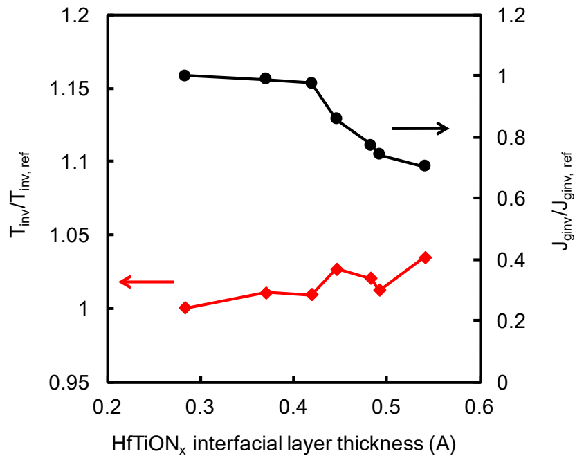
Figure 2-5 Normalized T_{\text{inv}} and J_{\text{ginv}} vs. \text{HfTiON}_x interfacial layer thickness. WSA was done at T_2 temperature.
