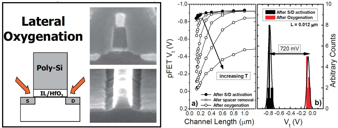
Figure 1-12 (left) Concept of lateral oxygenation. (right) pFET V_T as a function of channel length. Oxygenation anneal can reduce pFET V_T at shorter gate length, but the effect of anneal becomes smaller with longer gate length [25].
