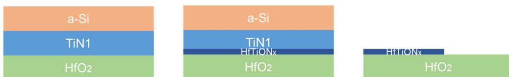
Figure 2-13 Schematics for possible multi- V_T integration using eWF control technique discussed in this work. (A) a-Si/TiN1 removal prior to WSA, (B) \text{HfTiON}_x removal after WSA.
