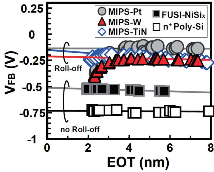
Figure 1-10 V_{fb} as a function of EOT. V_{fb} roll-off behavior was observed for high WF metal [32].
