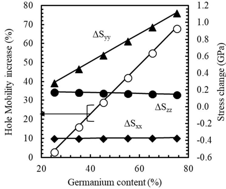
Figure 4-12 Hole mobility change of IF-Si 1-x Ge x channel pFET (with eSiGe stressor) between channel width of 1 \mu m and 0.1 \mu m calculated from \Delta S_{xx} , \Delta S_{yy} , and \Delta S_{zz} (plotted together) in Figure 4-11 and piezo-resistance coefficient in ref [69] (Si 0.55 Ge 0.45 ).
