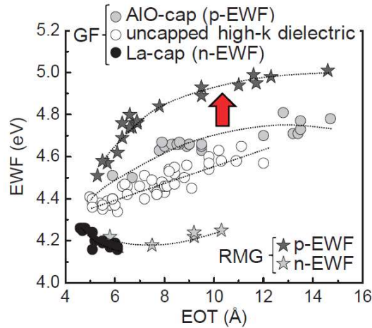
Figure 1-15 eWF as a function of EOT comparing gate-first and gate-last (from [39]).
