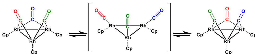
Scheme 1-5-1. Modified Merry-Go-Round 機構
