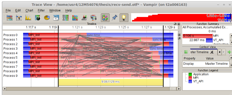
Figure A.1: Comparative Vampir visualizations | A graphical comparison of the performance of a collective vs. point-to-point operations to perform the same data exchange pattern.
