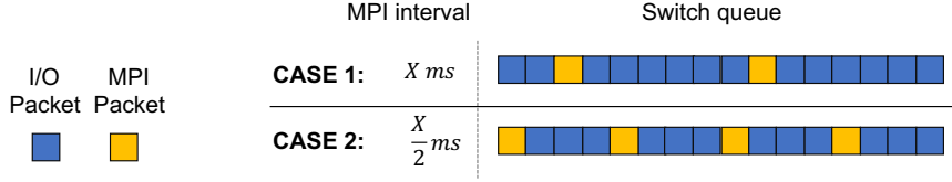
Figure 5.6: Expected state of switch queues when MPI interval is reduced by half.
