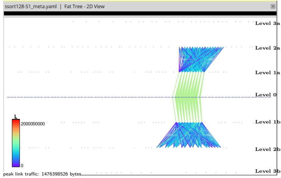
Figure 4.6: Boxfish visualization of samplesort ’s communication traffic after using a different node set | The nodes in the new set are in close physical proximity to each other. Notice that no traffic is going to level 3 switches, and hence those links are not visible.
