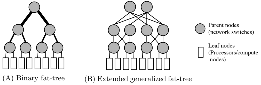
Figure 4.1: Fat-tree topologies Line thickness indicate the link’s relative capacity.
