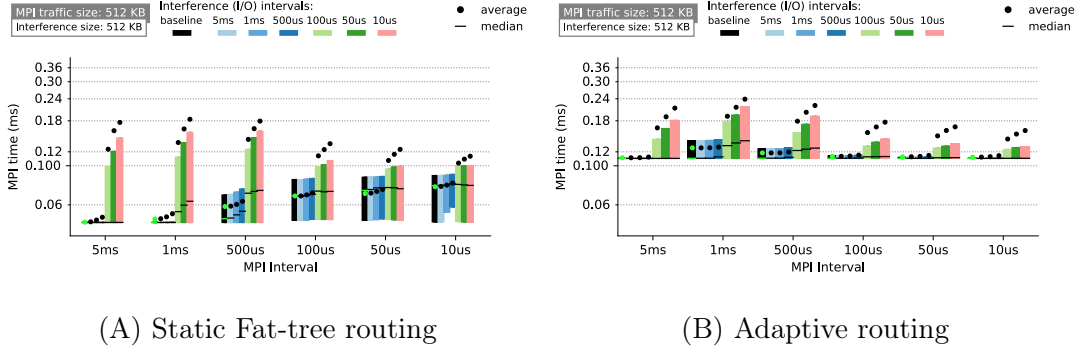
Figure 5.9: MPI performance with different routing algorithm
