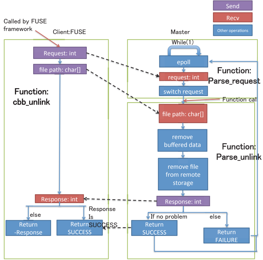
Figure 3.20: Process of unlink
