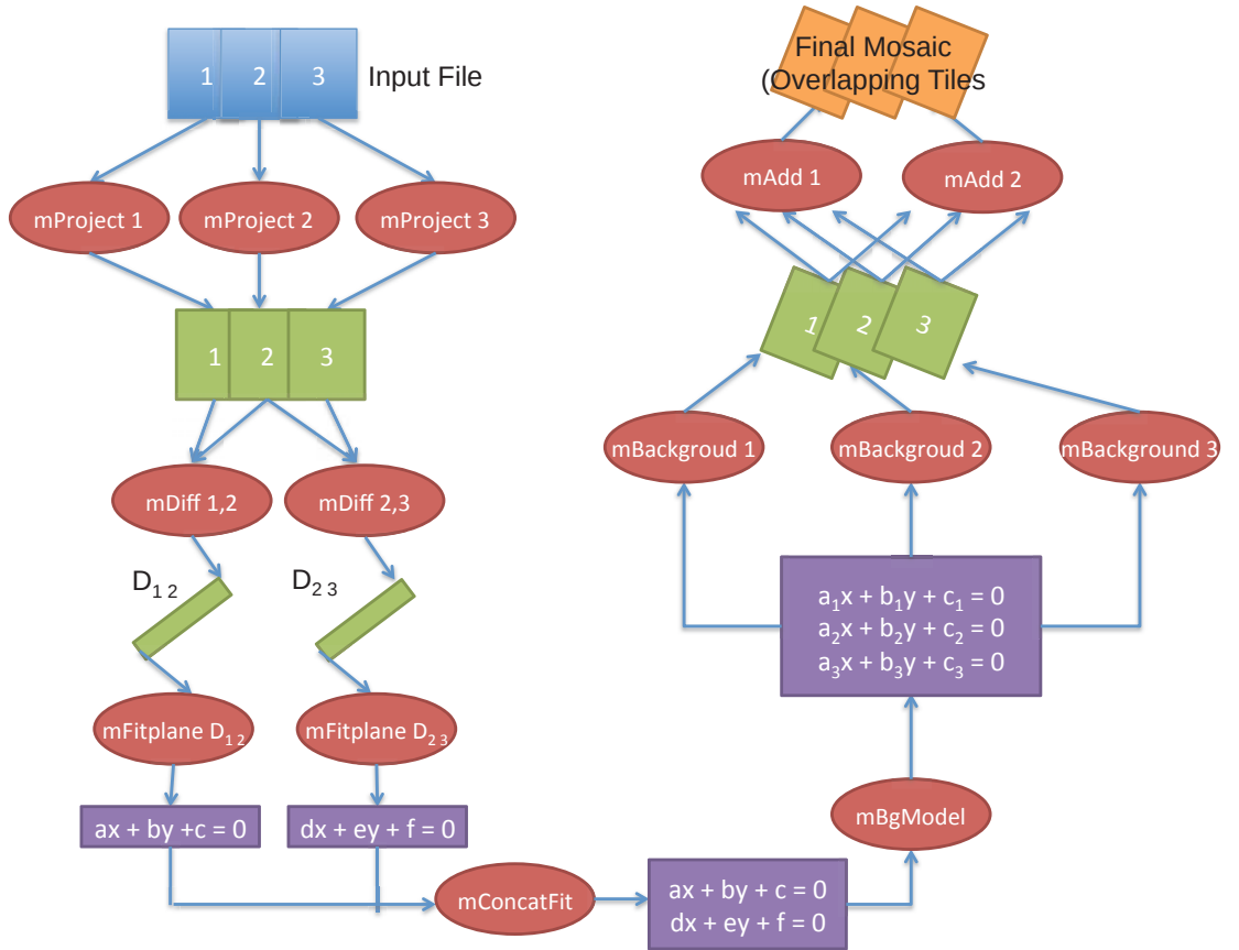
Figure 2.1: The Process of Montage [14]
