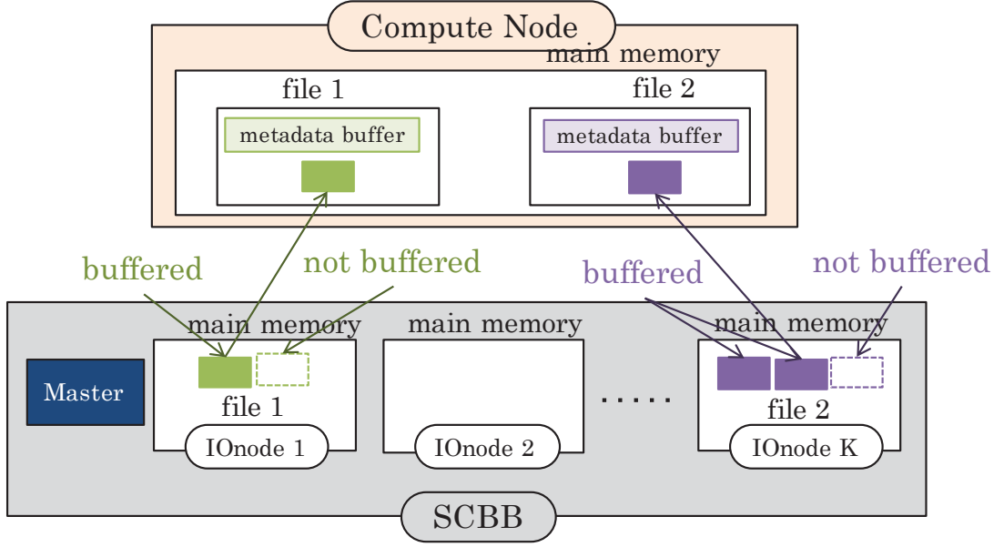
Figure 3.2: File Chunking and Buffers in Compute Nodes
