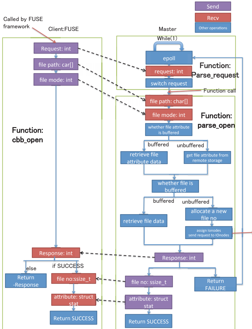
Figure 3.13: Process of open/create file
