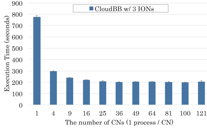
(a) Execution time of BT-IO using three IONs (Strong Scaling)
