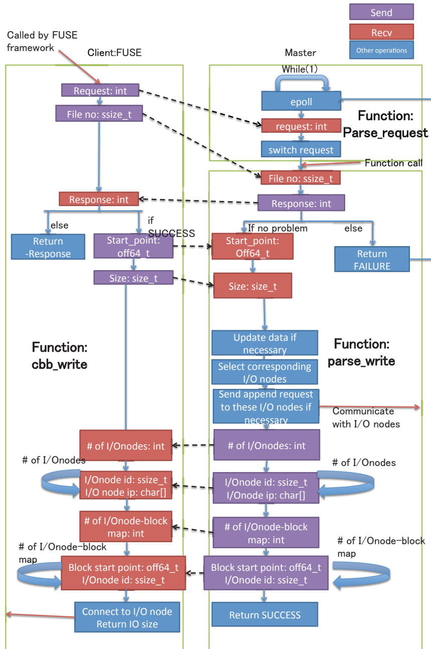
Figure 3.14: Process of Write
