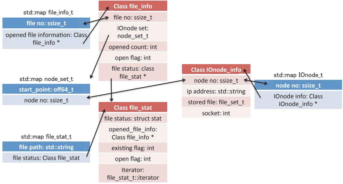
Figure 3.4: Data Structure in Master
