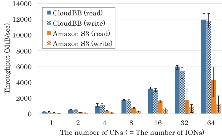
(a) Sequential I/O performance
