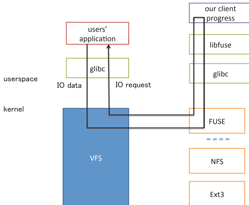
Figure 2.18: FUSE Architecture
