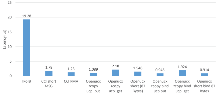
Figure 4.2: The Latency Comparison between TCP/IP and RDMA
