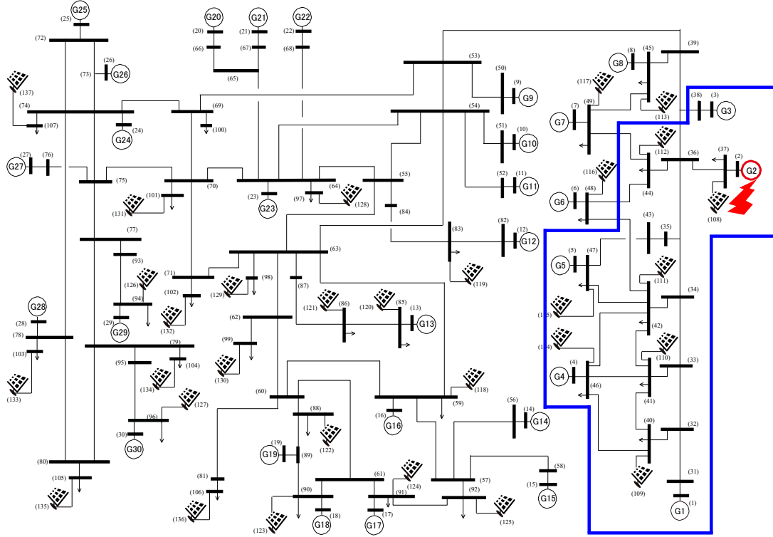
Fig. 4.3 PV-integrated IEEJ EAST 30-machine power system.
