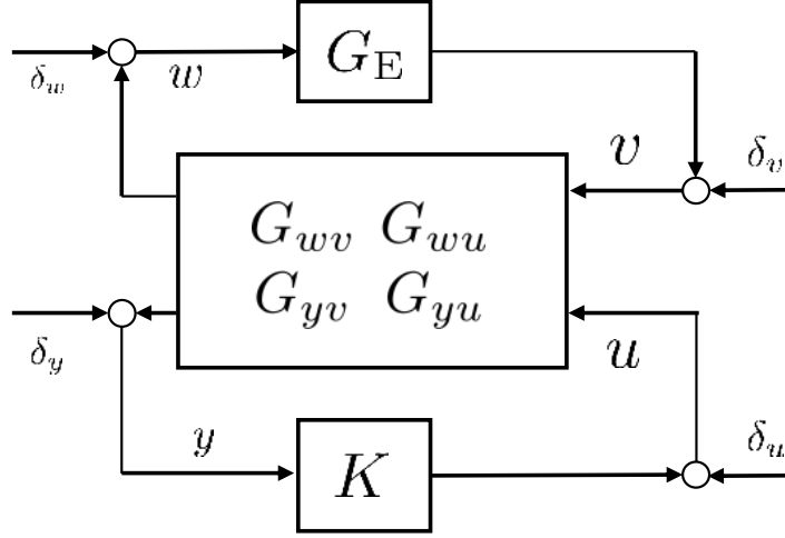
Fig. 2.3 An equivalent system to that in Fig. 2.2 for stability analysis.
