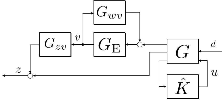
Fig. 2.6 Block diagram of the closed-loop map with an output-rectifying retrofit controller.
