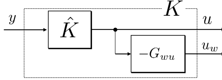
Fig. 2.7 Structure inside the input-rectifying retrofit controllers under full-control for the interconnection signal.
