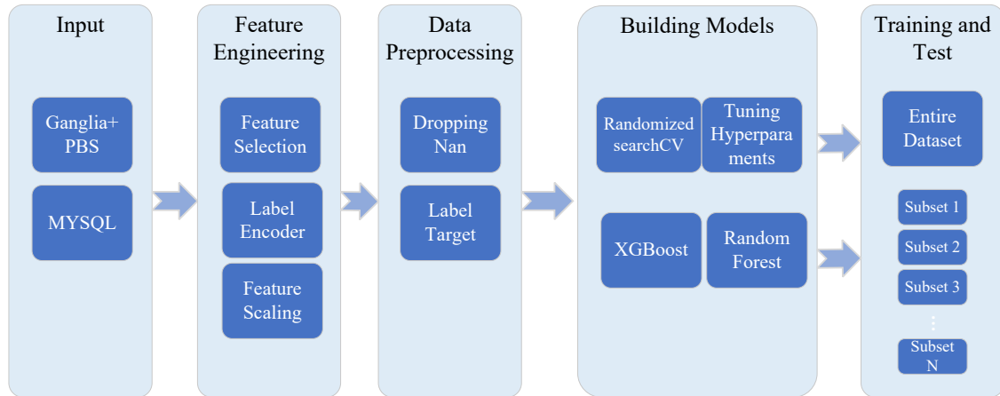
Figure 4.2: Overall Workflow about How to Build Machine Learning based Models
