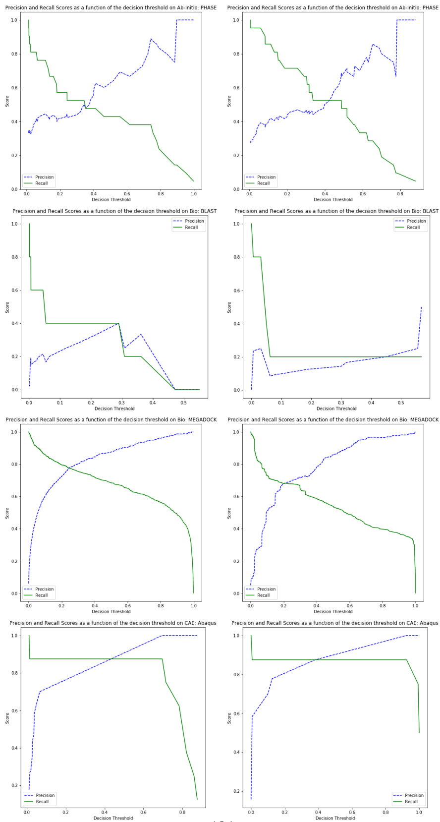
Figure A.1: Precision and Recall as Function of Threshold by XGBoost (Left) and Random Forest (Right) for Different Applications
