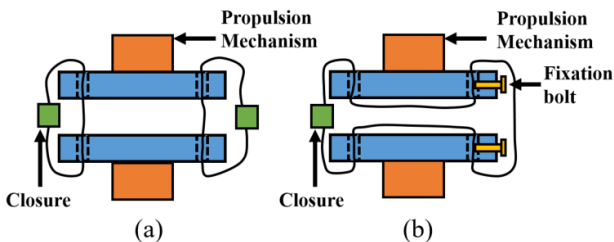
Fig.3 Attachment mechanism. (a) Modified pin belt. (b) Modified NATO belt.
