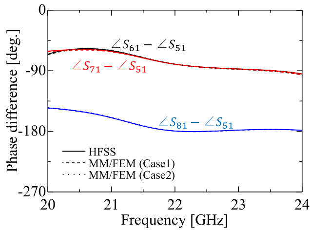
Fig. 6 Phase differences in the 2-plane hybrid coupler.
