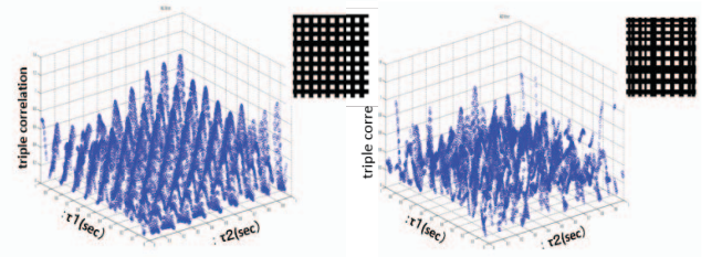
Fig. 2. Distribution of triple correlation values a) Normal triple correlation b) AD triple correlation
