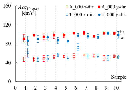
Fig. 6 Max. acceleration at 10th story
