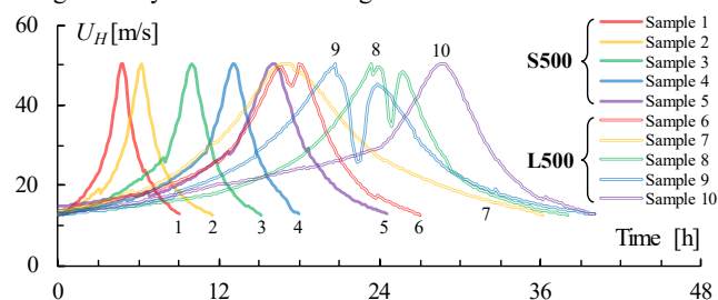
Fig. 3 Average wind speed
