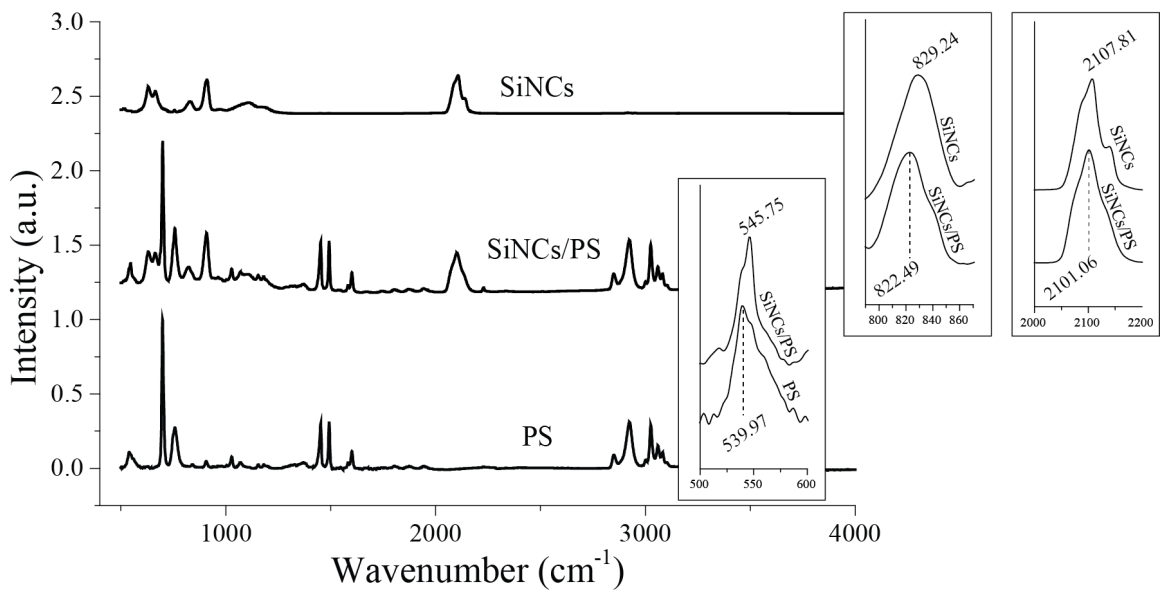
Figure 2-8 FT-IR spectrum of SiNCs, PS, and SiNCs/PS nanocomposite
