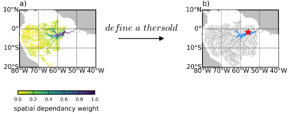
Figure 4.2 : Schematic diagram of the delineation of the empirical local patch for the target pixel indicated by a red star. (a) Spatial dependency weights and (b) local patch. River pixels inside the local patch are shown in blue, while other river pixels are shown in grey.
