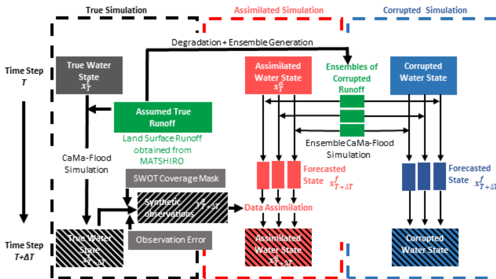
Figure 5.1: General framework of the observing system simulation experiment (OSSE)
