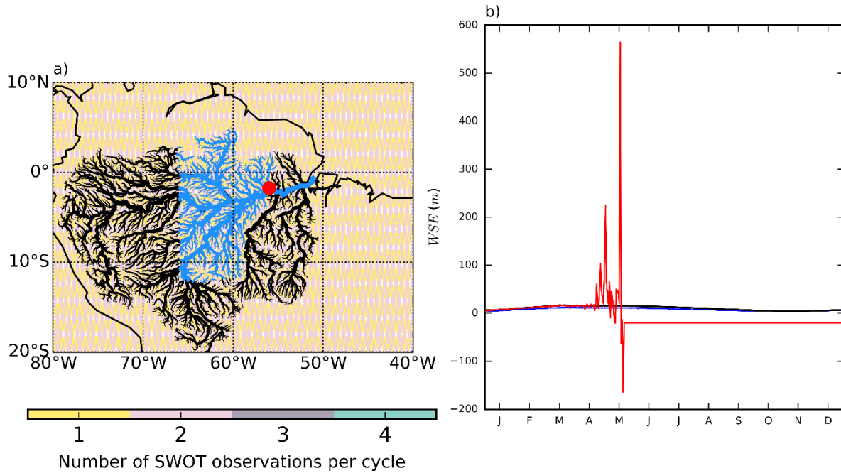
Figure 4.19 : a) Local patch with the number of SWOT observations (colours) and b) time series of WSE of Obidos. The Amazon River network is shown in black. Red circle indicates the target pixel.
