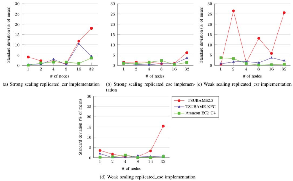
FIGURE 3.6: Performance variability for strong and weak scaling experiments with Graph500 replicated_csr and replicated_csc implementations on TSUBAME2.5, TSUBAME-KFC, and Amazon EC2 c4.8xlarge instances
