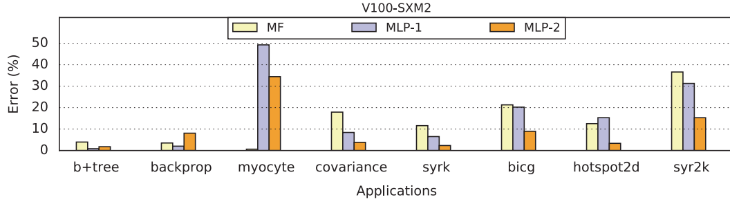
FIGURE 5.6: Evaluation of MF, MLP-1 and MLP-2 on V100-SXM2 GPU
