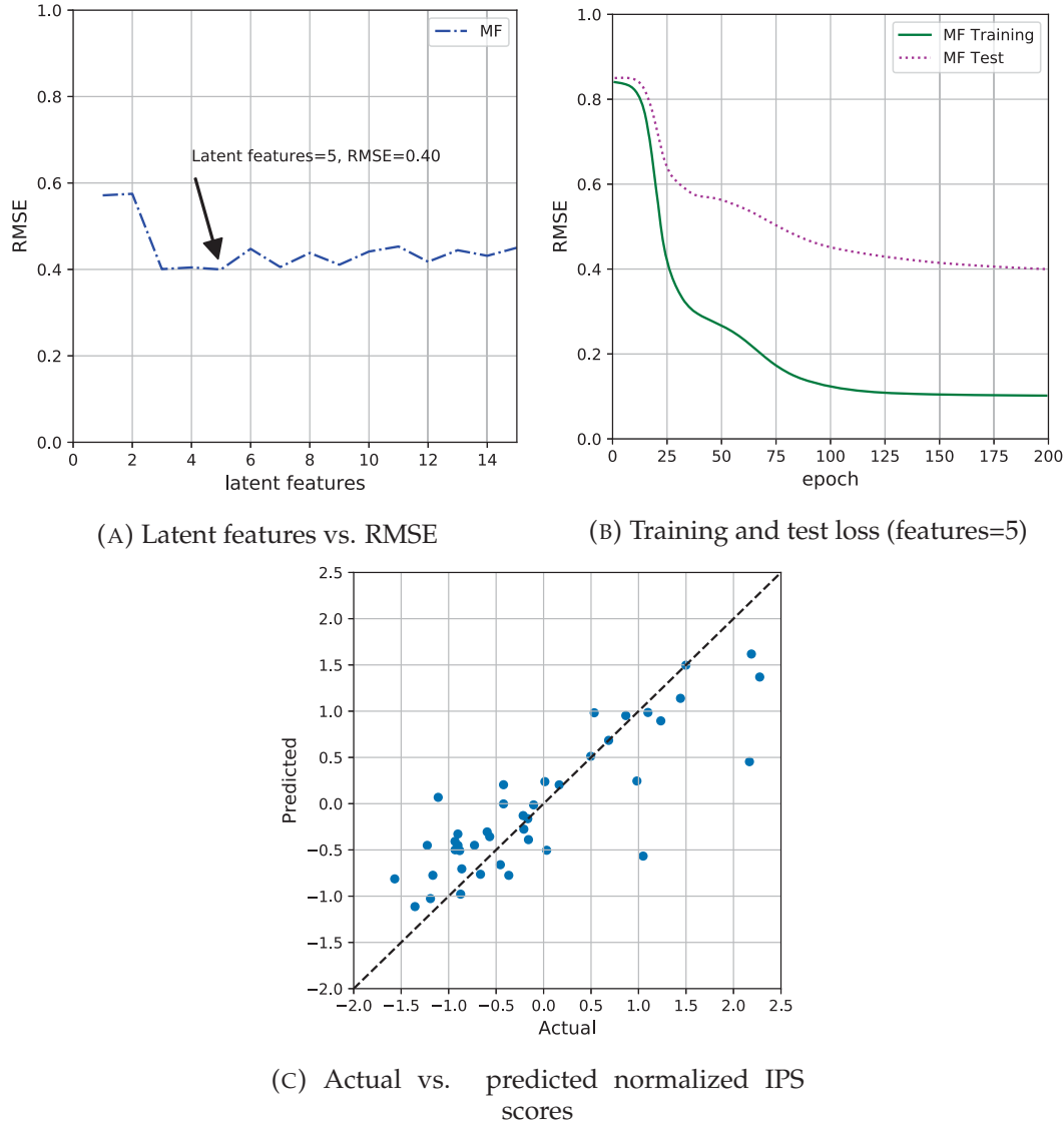
FIGURE 5.3: Prediction performance of matrix factorization using latent features with IPS dataset.
