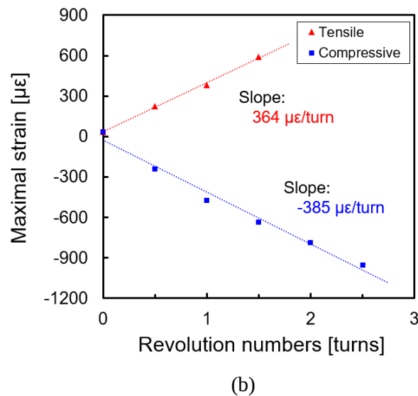
Fig. 5.5 (a) Strain distributions along the sensing fiber measured when the tensile strains of 0, 200, 400, and 600 \mu\epsilon and the compressive strains of 0, 200, 400, 600, 800, and 1000 \mu\epsilon were applied. The dotted lines indicate the theoretical trends. (b) Maximal tensile and compressive strains (derived from (a)) plotted in terms of the revolution numbers of the top screw.
