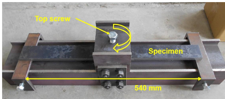
Fig. 5.4 Three-point bending device.
