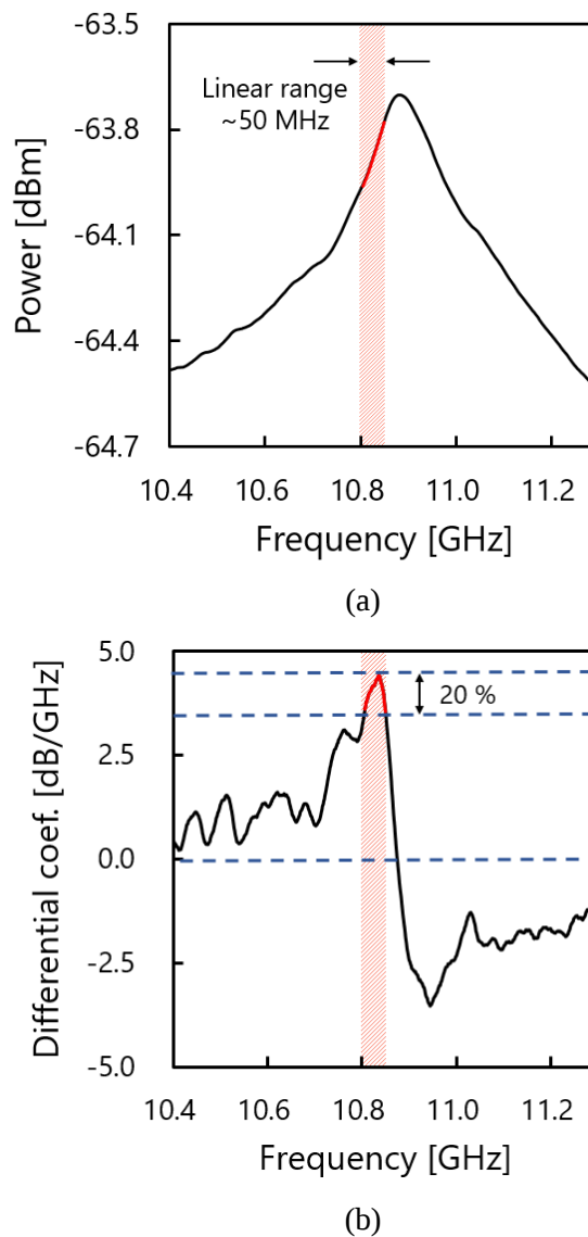
Fig. 2.2 (a) Measured BGS and (b) its differential coefficient at each frequency. Highlighted region indicates the linear region of the BGS (lower-frequency side is indicated).
