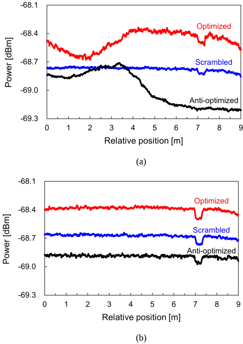
Fig. 4.9 Spectral power distributions along (a) the SMF and (b) the PMF measured at three different states of polarization, when 1000 \mu\epsilon strain was applied to the FUTs (7.0–7.3 m).
