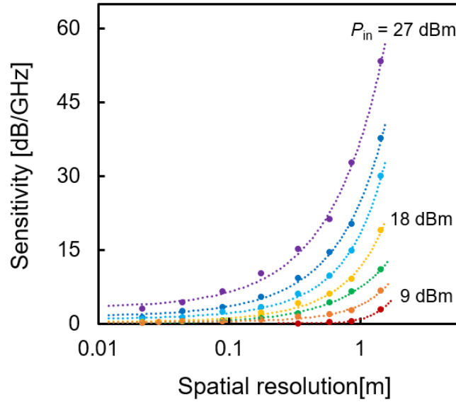
Fig. 3.13 Measurement sensitivities plotted as functions of the spatial resolution at incident powers from 9 to 27 dBm (step: 3 dB).
