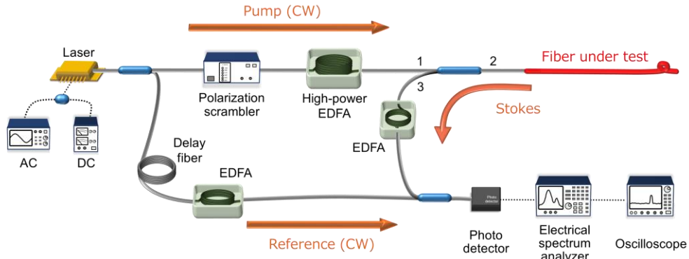
Fig. 4.12 Experimental setup of SA-BOCDR. AC, alternating current; CW, continuous wave; DC, direct current; EDFA, erbium-doped fiber amplifier.
