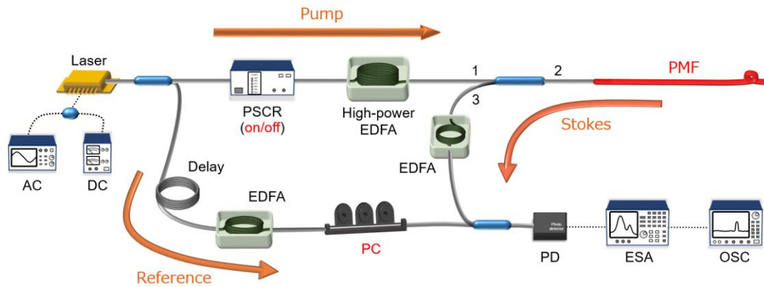
Fig. 4.8 Experimental setup of SA-BOCDR, in which the polarization scrambler (PSCR) can be switched on and off. EDFA, erbium-doped fiber amplifier; ESA, electrical spectrum analyzer; OSC, oscilloscope; PC, polarization controller; PD, photo diode; PMF, polarization-maintaining fiber.
