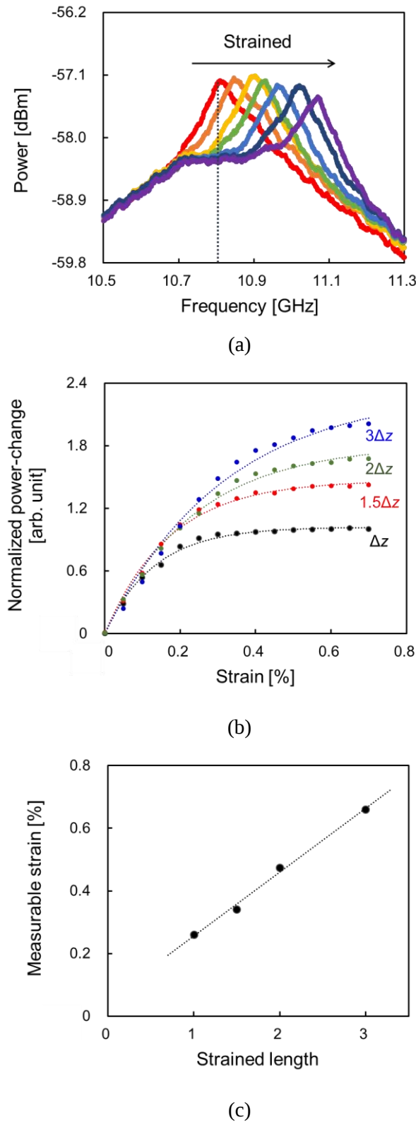
Fig. 4.15 (a) BGSs measured at strains of 0–0.6% (step: 0.1%) when the strained length L_e was 3\Delta z , where \Delta z is \sim 0.37 m. (b) Normalized power changes plotted as functions of applied strain when the L_e values were \Delta z , 1.5\Delta z , 2\Delta z , and 3\Delta z . The dotted curves are exponential fits. (c) Maximal measurable strain plotted as a function of L_e . The dotted line is a linear fit.
