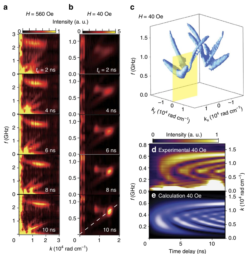
Figure 4 | Time-resolved SWaT spectra. (a,b) Time-resolved SWaT spectra with \mathbf{k} parallel to \mathbf{M} under in-plane magnetic fields of 560 Oe (a) and 40 Oe (b) respectively. The data was obtained by applying a time-window with the width of 2.8 ns centred at the time delay noted in each figure. (c) A three-dimensional contour plot (at the intensity of 0.97 in the scale shown in Fig. 2a) of the SWaT intensity obtained under the in-plane magnetic field of 40 Oe. The data shown in (b) was extracted along the cross-section shown as the yellow plane. (d) Temporal evolution of the time-resolved SWaT spectra obtained along the dashed white line in (b). The data was obtained by applying a time-window with the width of 1.0 ns. (e) A result of numerical calculations of the time-resolved SWaT spectra shown in (d).
