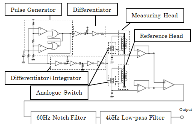
Fig. 4 MI sensor measurement system schematic diagram.
