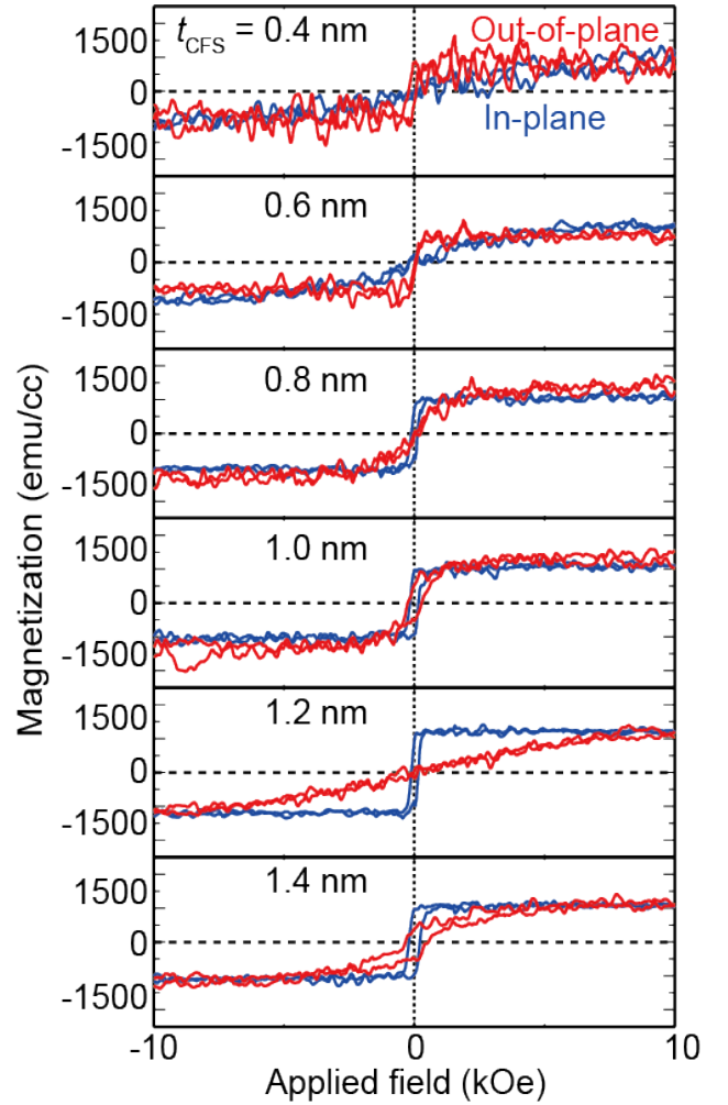
Fig. 4 Magnetization vs field curves for CFS/MgO bilayers formed at T_s = 350^\circ\text{C} . The thickness of the CFS layers were varied from 0.4 nm to 1.4 nm.
