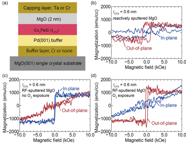
Fig. 1 (a) Schematic of a full stack of samples with a CFS/MgO bilayer. (b–d) M-H curves for CFS/MgO bilayers. The MgO layer was formed by (b) reactive sputtering and (c,d) RF sputtering. (d) The CFS surface was exposed to oxygen prior to RF sputtering of MgO layers. 9,10)
