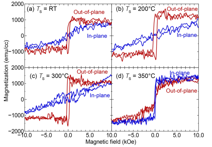
Fig. 2 M-H loops for CFS (0.6 nm)/MgO bilayers formed at (a) T_s = \text{RT} , (b) T_s = 200^\circ\text{C} , (c) T_s = 300^\circ\text{C} , and (d) T_s = 350^\circ\text{C} . The MgO layers were RF sputtered and the surface of CFS was exposed to an oxygen atmosphere.
