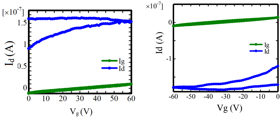
Figure 3.8: Transfer characteristics for (left) n-type transistor (right) p-type transistor at room temperature when V_d = 60 V for n-type and V_d = -60 V for p-type.
