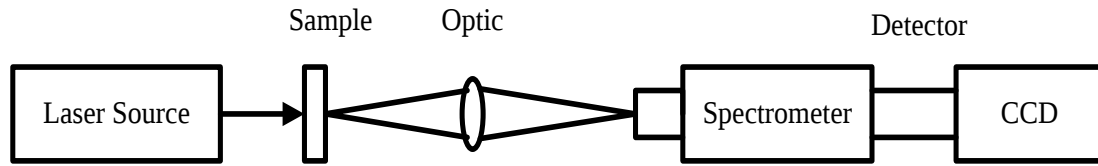
Figure 2.7: Schematic diagram of the photoluminescence setup [14].
