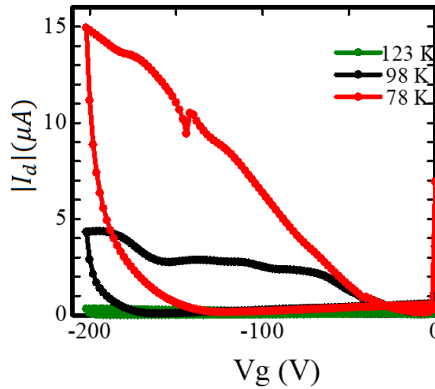
Figure 3.9: Transfer characteristics of two step fabricated film.
