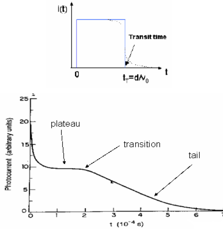
Figure 2.13: (top) Ideal photocurrent with tail due to circuit reaction time (bottom) measured photocurrent with long tail [31].
