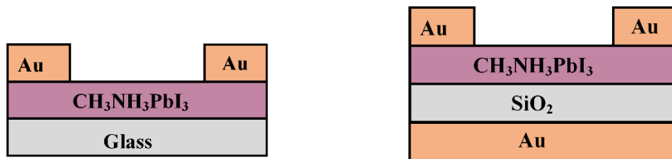
Figure 2.1: Perovskite structure (a) on the glass substrate and (b) silicon substrate
