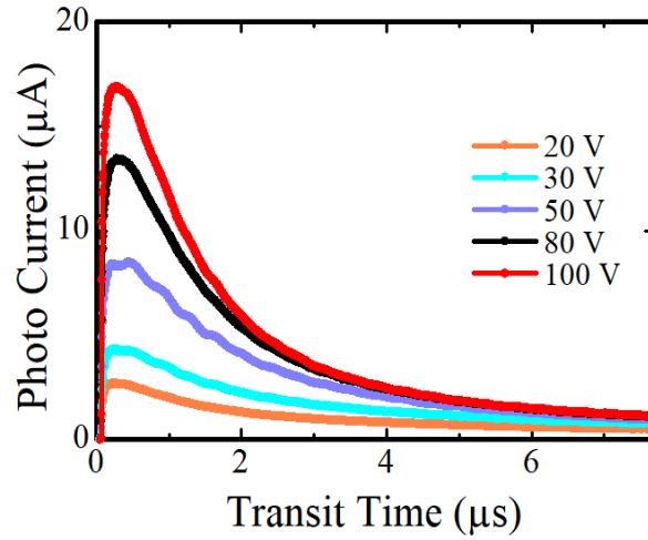
Figure 3.16: Two step voltage dependence TOF measurement.
