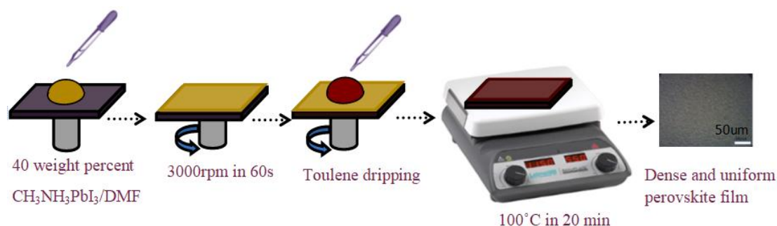
Figure 2.2: One-step spin coating process for perovskite thin film
