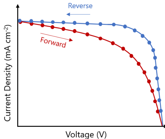
Figure 1.3: Current-voltage hysteresis encountered in perovskite solar cells.
