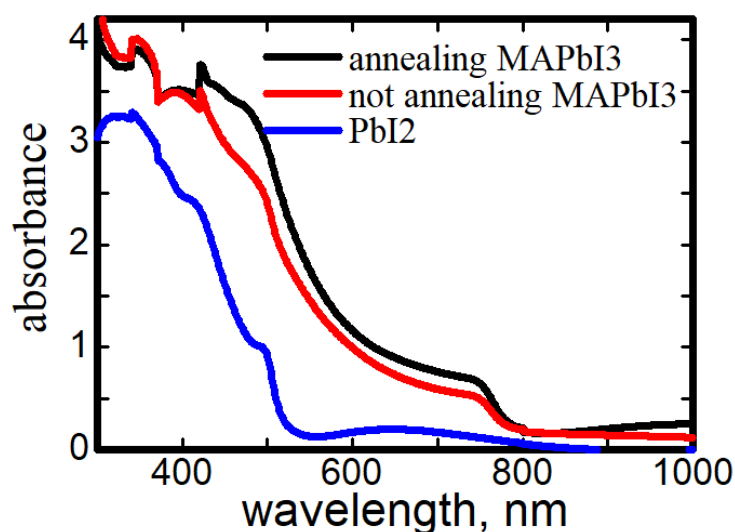
Figure 2.6: Absorbance spectrum for \text{PbI}_2 and \text{MAPbI}_2 film annealing and not annealing after reaction with MAI salt.
