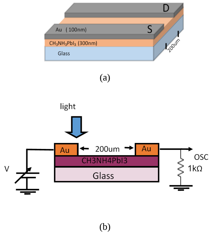
Figure 3.11: (a) Structure of perovskite thin film device for TOF measurement (b) electrical connection of the fabricate film for lateral TOF measurement.
