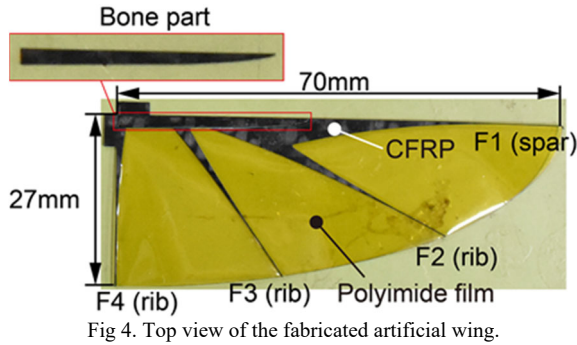
Fig 4. Top view of the fabricated artificial wing.
