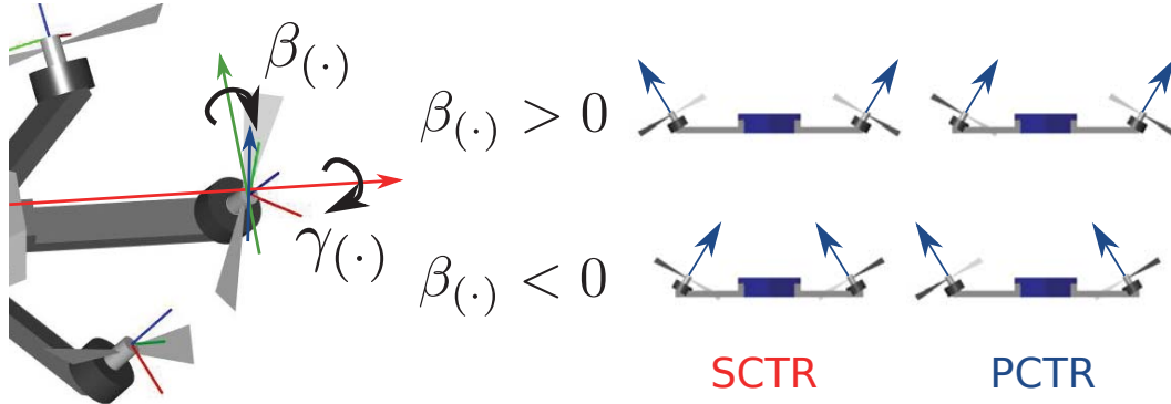
Fig. 3.5: Rotor tilt angles. Rotors are tilted in two axes, and the angles are denoted by \beta_{(\cdot)} and \gamma_{(\cdot)} . \beta_{(\cdot)} is the inward/outward angle, and \gamma_{(\cdot)} is the sideward angle. The rotation direction of \beta_{(\cdot)} is different among the two classes of hexarotor structures.
