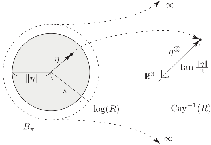
Fig. 2.3: Relation of \log(R) and \text{Cay}^{-1}(R) . The conversion from the axis-angle representation to the Cayley parameter corresponds to stretching of an open ball to \mathbb{R}^3 .
