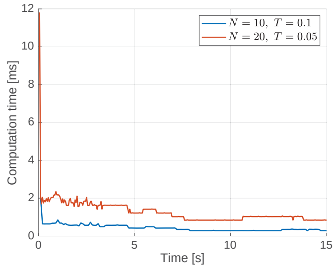
Fig. 5.6: Computation time for each sampling period (Simulation 5A). The proposed NMPC method is feasible in real time on a Raspberry Pi single-board computer.
