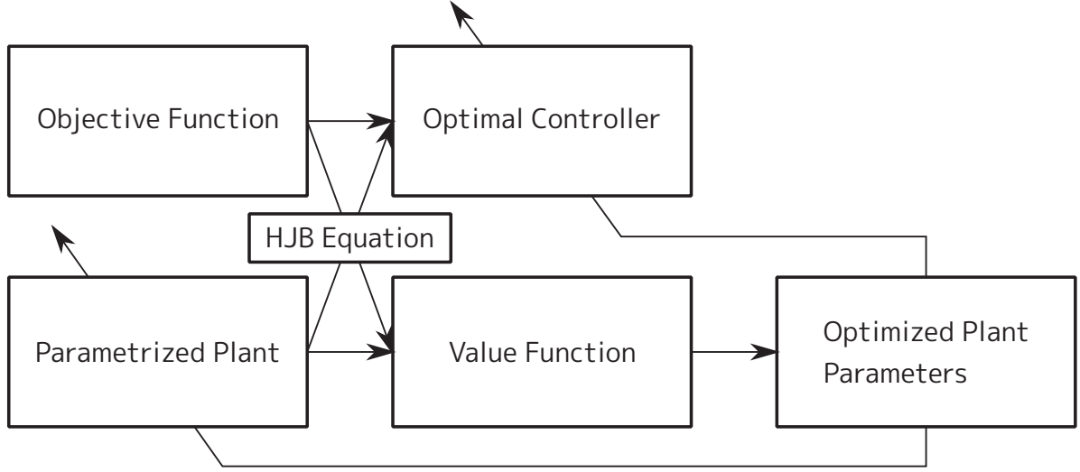
Fig. 4.1: Schematic of analytic joint optimization
