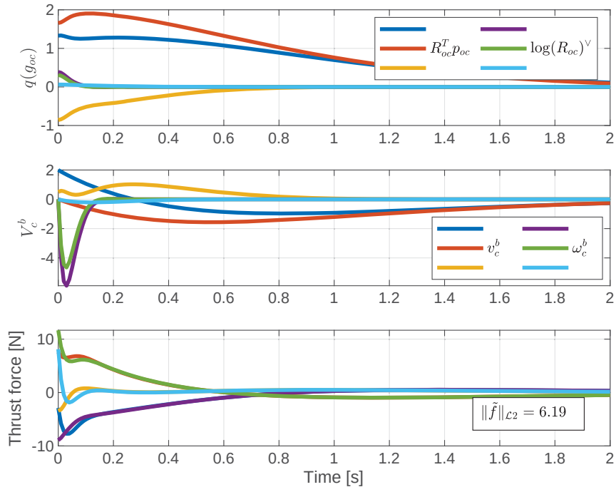
Fig. 4.5: Simulation 4B: The thrust force is larger than that of Simulation 4A (Fig. 4.4). The rate of convergence is also slower due to the poor ability of horizontal acceleration.
