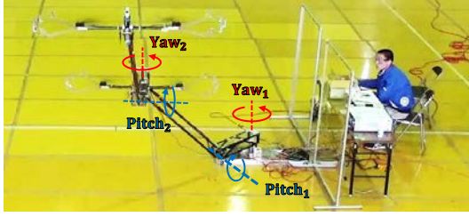
Fig.2 Overview of the prototype "Hiryu-II"
