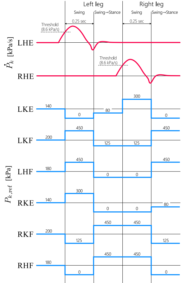
Fig. 8: State diagram of assist control
