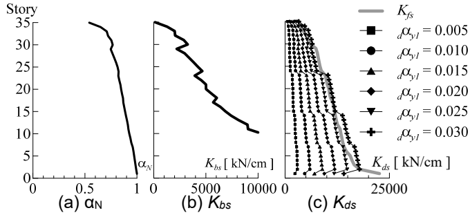
Fig.3 Frame parameters for control
