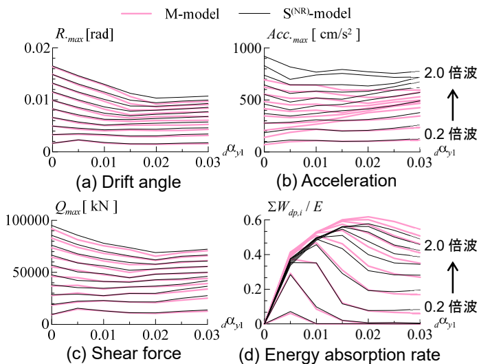
Fig.5 Response comparison between M-model and S^{(NR)} -model
