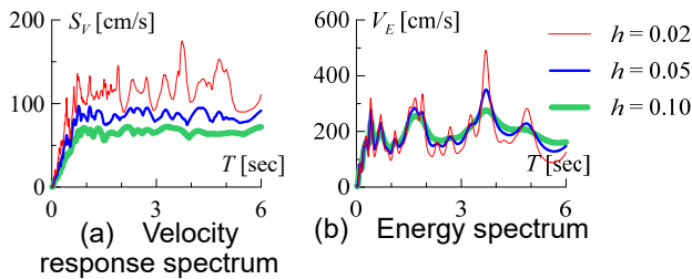
Fig.4 Earthquake spectrum
