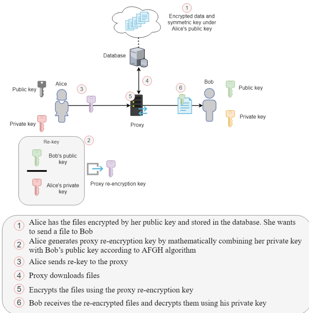
Figure 18: The proxy re-encryption scheme
